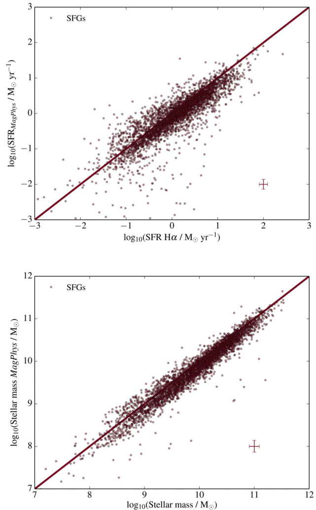
Figure B1. Top: The distribution of M_{\text{AGPHYS}} best-fitting estimates of SFRs of SFGs in the sample versus their H\alpha -SFRs. The solid black line shows the one to one relation in both panels. Bottom: The distribution of M_{\text{AGPHYS}} best-fitting estimates of stellar masses of SFGs in the sample versus their stellar masses given in the MPA-JHU catalogue.
