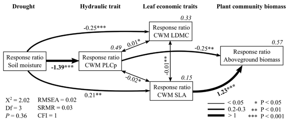
Figure 5. Minimal adequate structural equation model for the effects of soil moisture RRs on the linkages between CWM hydraulic trait RR (PLCp: percentage loss of hydraulic conductance), leaf economic trait RRs (SLA: specific leaf area; LDMC: leaf dry matter content) and above-ground biomass RRs to drought at Site 2 (Saint-George). The model highlights indirect effects of soil moisture reduction on above-ground biomass through changes in PLCp and SLA. Arrows show significant relationships (pathways) between variables and numbers next to arrows show standardized parameter estimates (i.e. standardized regression weights). Square multiple correlations ( R 2 values) for the predicted/dependent factor are given on the box of the dependent variable.
