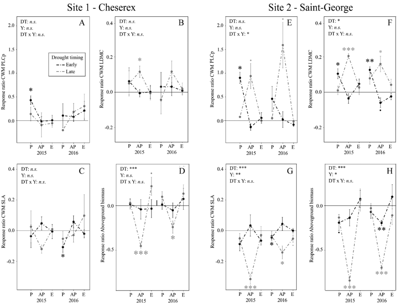
Figure 3. Response ratio of CWM plant traits [PLCp: predicted percentage loss of hydraulic conductance (A, E), LDMC: leaf dry matter content (B, F), SLA: specific leaf area (C, G)] and biomass production (D, H) to early- (Early; black circle) and late-season drought simulation (Late; grey circle) along the plant growing season (P: Peak, AP: After peak, E: End) at both sites and for both years. Within each year Peak and After peak, as well as After peak and End, are separated by 2 months. Statistical results are displayed for the effects of the timing of drought (DT: Early vs. Late), the year (Y: 2015 vs. 2016) and their interaction (DT × Y) and indicated for RRs significantly different from zero. Significant effects are indicated in each graph ( P < 0.10 , *P < 0.05 , **P < 0.01 , ***P < 0.001 ).
