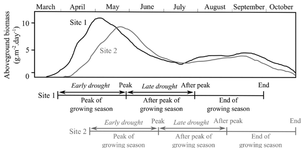
Figure 1. Scheme of the seasonal dynamic of grassland biomass production for the two sites (unpublished data available from Agroscope institute). The different periods of plant growth along the season (each lasting for 2 months) are represented below the graph (Peak of growing season, After peak of growing season and End of growing season) with their respective sampling times (Peak, After Peak and End) for plant trait measurements and above-ground biomass harvest. The ‘peak of growing season’ period has been centred on the peak of the vegetation growth curve and determined the beginning of the experiment at each site. The growth curve, periods and sampling times are drawn in black for Site 1 and grey for Site 2. Drought was applied either during the peak of growing season (i.e. Early drought) or after the peak of growing season (i.e. Late drought). Mowing occurred at the sampling times (Peak, After Peak and End) to simulate common management practices at both sites.
