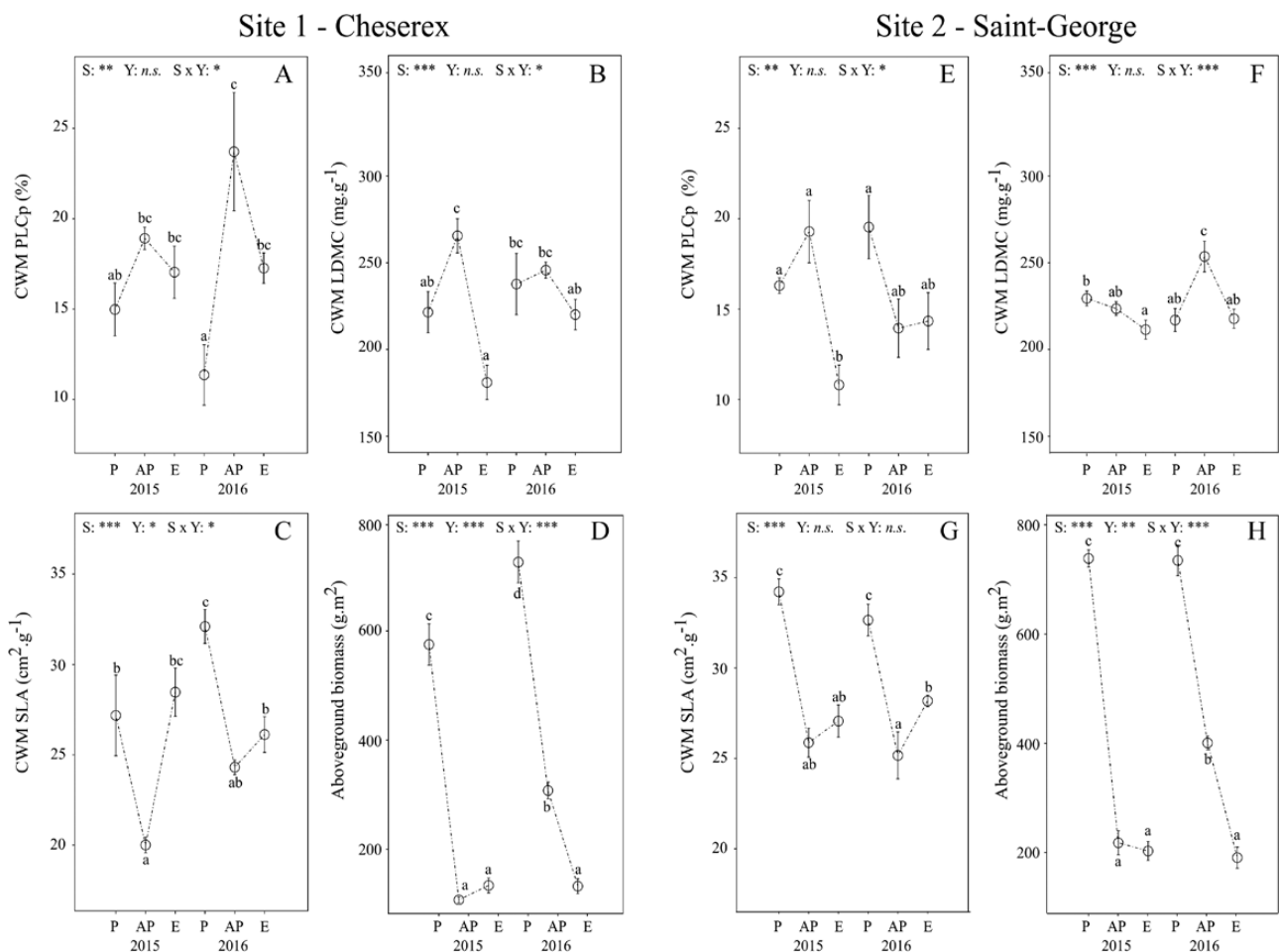
Figure 2. Seasonal and inter-annual variability in CWM plant traits [PLCp: predicted percentage loss of hydraulic conductance (A, E), LDMC: leaf dry matter content (B, F), SLA: specific leaf area (C, G)] and biomass production (D, H) along the plant growing season (P: Peak, AP: After peak, E: End) at both sites and for both years. Within each year Peak and After peak, as well as After peak and End, are separated by 2 months. Statistical results are displayed for the effects of the season (S: Peak, After peak, End), the year (Y: 2015 vs. 2016) and their interaction (S \times Y) and significant effects are indicated in each graph (** P < 0.05 , *** P < 0.01 , **** P < 0.001 ).
