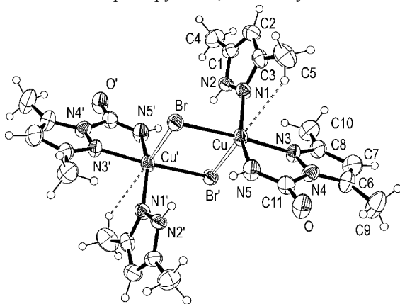
Fig. 1. ORTEP drawing of complex [CuBr(HL 1 )(L 3 ) 2 ] with atom numbering scheme.
