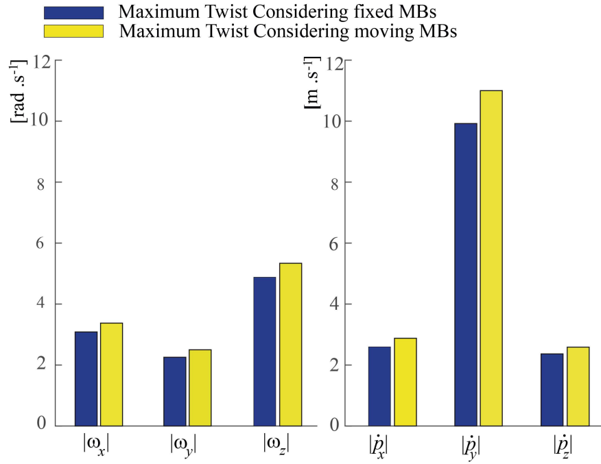
Fig. 13 Kinematic performance of FASTKIT
