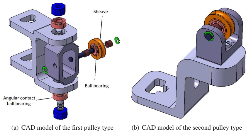
Fig. 5 FASTKIT pulleys
