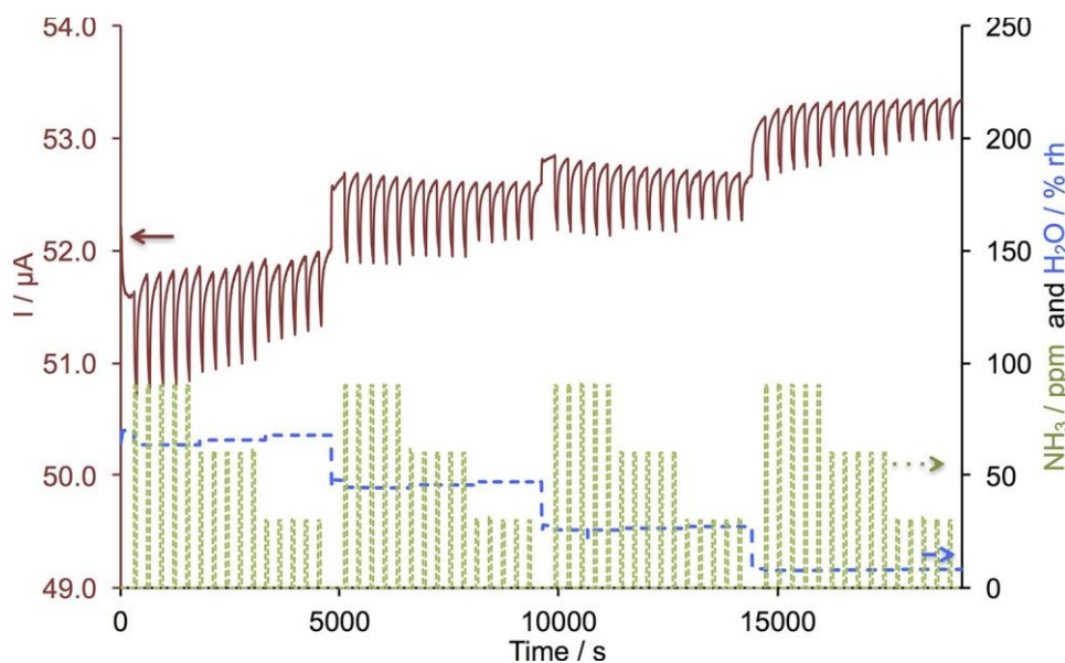
Figure 5: Response of a MSDI 2 (solid line) to \text{NH}_3 (90, 60 and 30 ppm, dotted line), with relative humidity in the range 10-70 % (dashed line), during exposure/recovery cycles (1 min/4 min); T = 20^\circ\text{C} .
