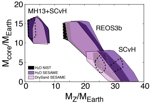
Fig. 10. Space of solutions obtained with different equations of state for H and He and for heavy elements. Solutions with REOS3b shifted to lower masses of heavy elements. We obtain fewer solutions with SCvH.
