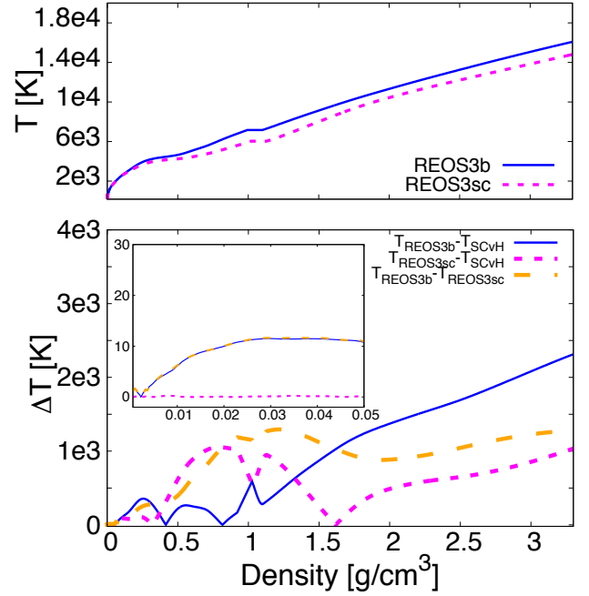
Fig. 12. Jupiter's structure with REOS3sc. It has lower temperatures than in Miguel et al. (2016) and is much closer to the profile obtained with SCvH for lower densities.
