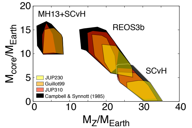
Fig. 8. Mass of the core and heavy elements in the interior of Jupiter derived with different J_s . The ranges of core masses are the same as those in Miguel et al. (2016) for SCvH and MH13, and the lower limit changed from 7 to 5 M_\oplus for REOS3b. The mass of heavy elements that we get when using REOS3b is smaller in all cases.
