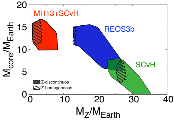
Fig. 9. Areas in the mass of the core and heavy elements space correspond to solutions found with different equations of state: SCvH (green), MH13+SCvH (red) and REOS3b (blue area). The space of solutions obtained with REOS3b has shifted towards solutions with a lower mass of heavy elements compared with Miguel et al. (2016). We also find fewer solutions that have a high mass of heavy elements for SCvH. The range of solutions for the core mass remain unchanged for SCvH and MH13 and for REOS3b the lower limit is 5 M_{\oplus} compared with 7 M_{\oplus} before.
