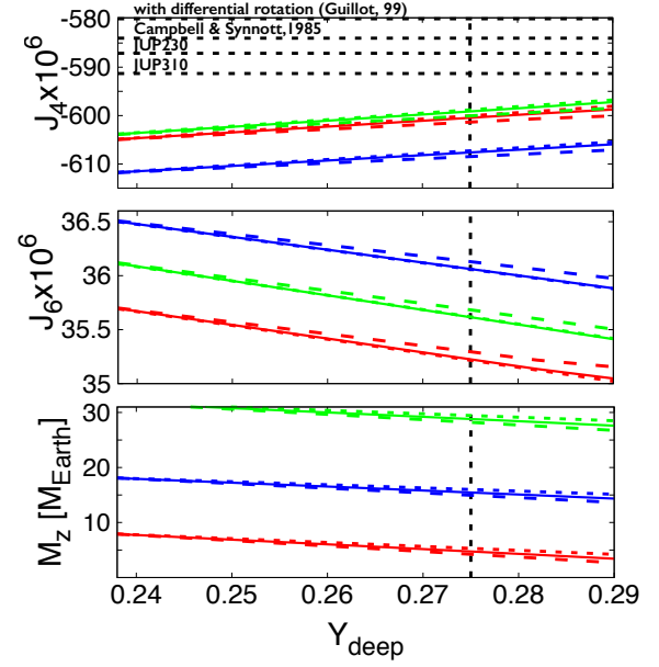
Fig. 7. Heavy element masses. The main differences compared with the previous results is the change in J_6 and the mass of heavy elements. The mass of heavy elements with REOS3b is smaller than in the previous results.
