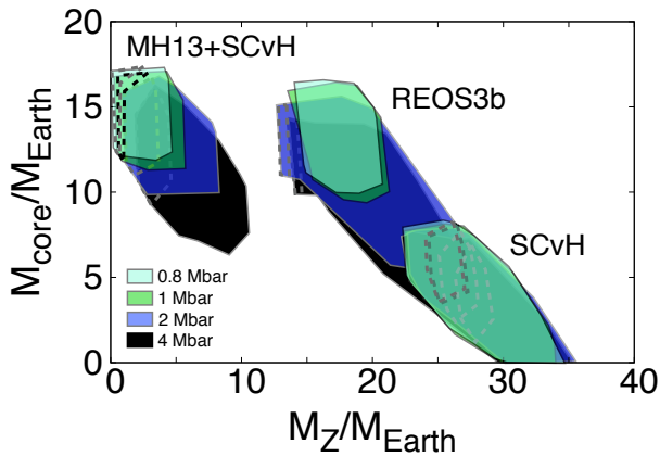
Fig. 11. Results of optimization models with different equations of state for H and He and changing the location of the P_{\text{Sep}} : 4 Mbar (black), 2 Mbar (blue), 1 Mbar (green), and 0.8 Mbar (light blue). As in previous figures, solutions with REOS3b have a lower mass of heavy elements. When using a P_{\text{Sep}} = 4 Mbar and REOS3b, we find lower core masses that go as low as 2 M_{\text{Earth}} .
