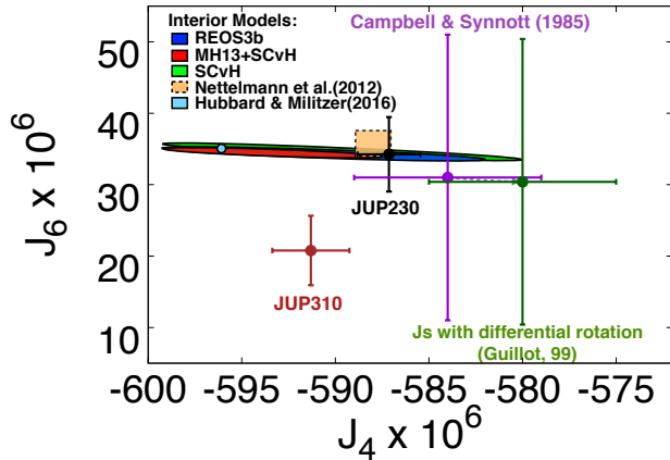
Fig. 6. Values of the gravitational moments J_4 and J_6 . This figure includes an up-to-date calculation of the model J_4 and J_6 (see text). It was rotated in order to adopt the same convention as other publications (e.g. Bolton et al. 2017).
