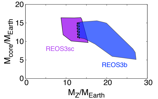
Fig. 13. Range of core masses and mass of heavy elements. This range has changed for both EOS. For REOS3b see previous figures and main text, for the case of REOS3sc, the new ranges are M_{\text{core}} 10\text{--}17 M_{\oplus} and M_Z 8\text{--}16 M_{\oplus} , compared to M_{\text{core}} 7\text{--}17 M_{\oplus} and M_Z 13\text{--}32 M_{\oplus} in previous calculations.
