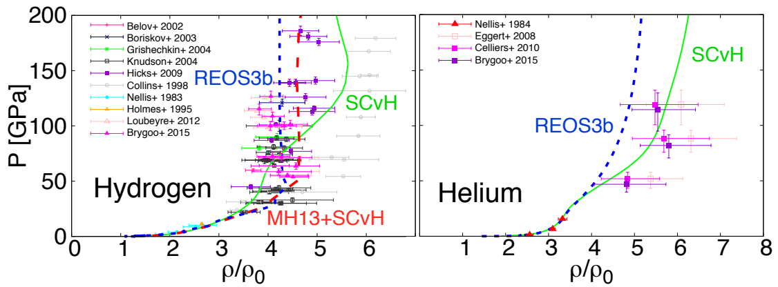
Fig. 4. Principal Hugoniot of hydrogen ( left panel ) and helium ( right panel ). Due to the small changes in the EOS there is no visible change in the Hugoniot curves.
