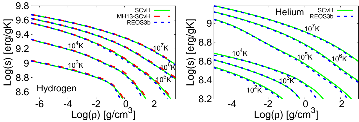
Fig. 3. Specific entropy vs. density at different temperatures for hydrogen ( left panel ) and helium ( right panel ). Given the small changes in the EOS, the differences between this figure and Fig. 3 in Miguel et al. (2016) are not visible.
