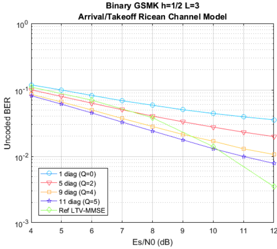
Fig. 6. Comparison with the LTV-MMSE [10]
