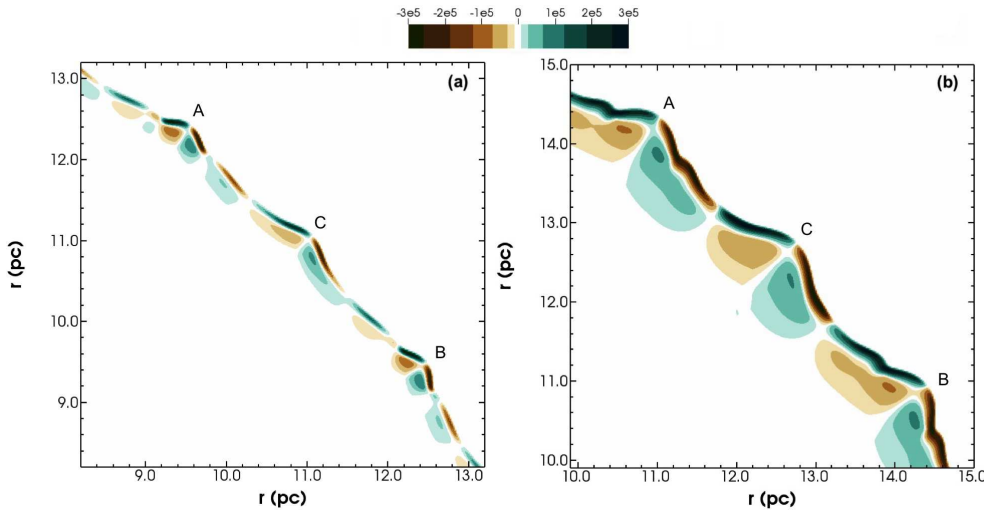
Fig. 10. Transverse mass flux ( \rho v_r ) map; panel a : at t \approx 58 \text{ kyr} , panel b : at t \approx 93 \text{ kyr} . We clearly see transverse fluxes in the dense shell, from the hills to the valleys, characteristic of the VI mechanism. They are still active at a very advanced age.
