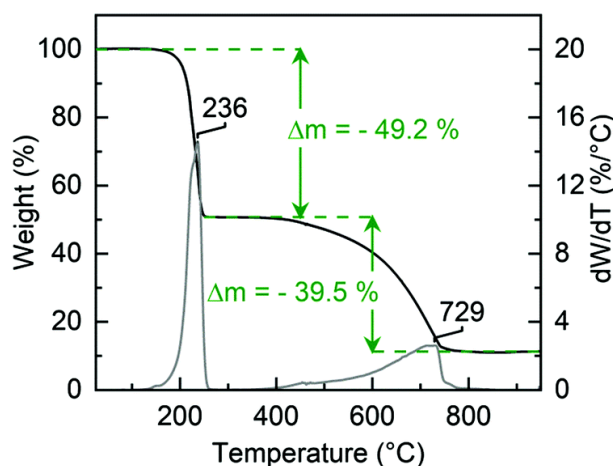
Fig. 2 TGA trace (black) and its first derivative (grey) of CP2 under Ar atmosphere in the range of 25 to 950 °C. Scan rate = 10 °C min −1 .
