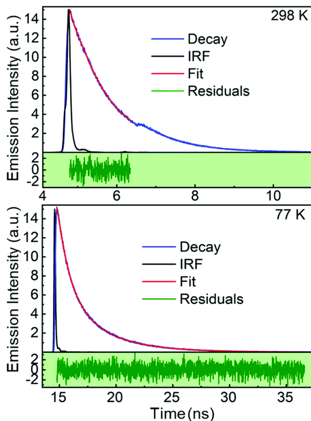
Fig. 6 Emission decays of CP2 (blue), fit (red), IRF (black) and residual (green) using a nano-LED laser ( \lambda_{\text{exc}} = 378 nm; fwhm = 90 ps; power = 0.45 pJ) at 298 K ( \tau_{e1} {f%} = “0.03” ns {3.0}; \tau_{e2} {f} = 0.93 ns {97.0}, \chi^2 = 1.16 ) and 77 K ( \tau_{e1} {f%} = 1.0 ns {32.6}; \tau_{e2} {f%} = 3.5 ns {67.4}, \chi^2 = 1.06 ). Note that this 0.03 ns value is not considered accurate due pulse width at half-maximum of the excitation source and its relative intensity (see footnote of Table 3).
