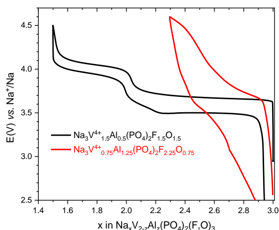
Figure R1: Comparison of the electrochemical profiles obtained for the sodium cells Na/Na_3V^{4+}_{1.5}Al_{0.5}(PO_4)_2F_{1.5}O_{1.5} and Na/Na_3V^{4+}_{0.75}Al_{1.25}(PO_4)_2F_{2.25}O_{0.75} .
