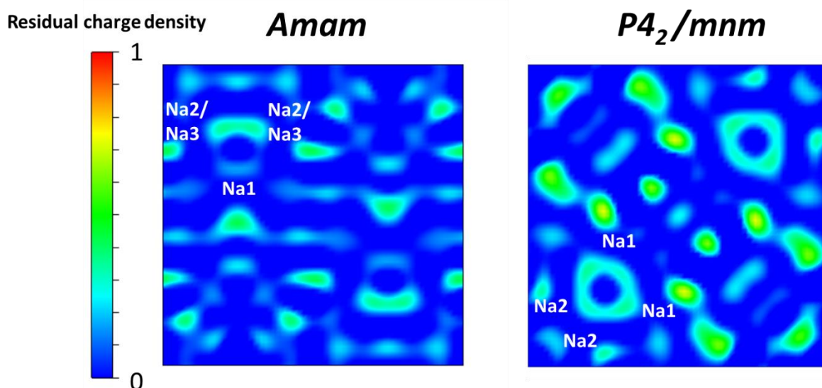
Figure S2. Fourier difference maps of \text{Na}_3\text{V}_{1.5}\text{Al}_{0.5}(\text{PO}_4)_2\text{F}_3 in the Amam and P4_2/mnm space groups.
