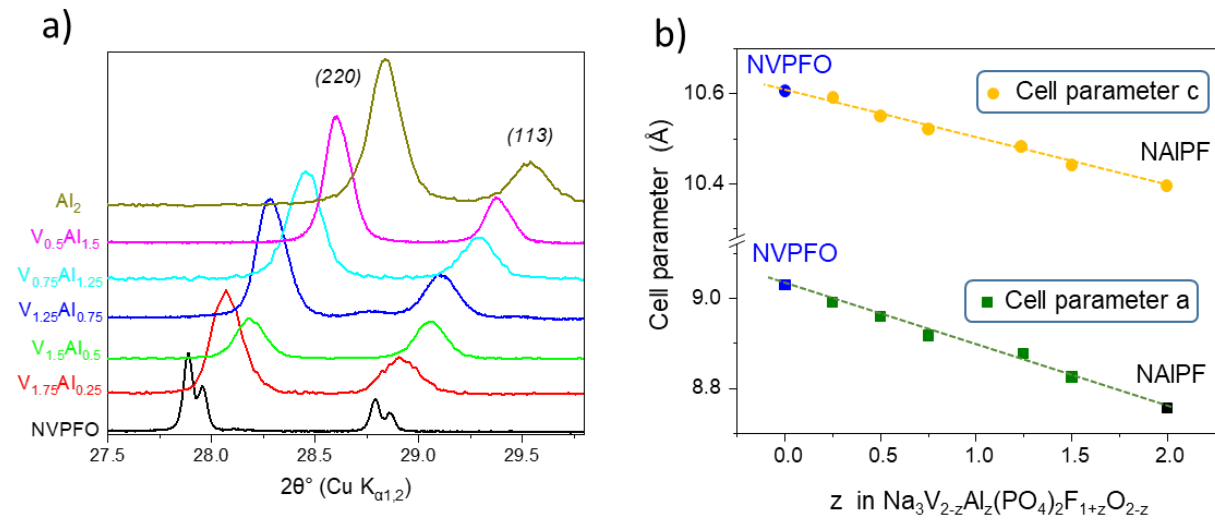
Figure S4 a) Enlargement of the powder XRD patterns given in Figure S3 between 27.5 and 29.6 °(2θ). The different V : Al ratio listed on the left were determined by ICP-OES analyses b) Evolution of the cell parameter a and c according to the Al for V substitution.
