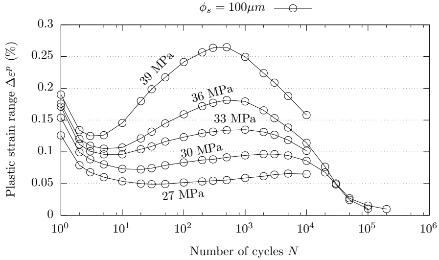
Figure 4: Evolution of \Delta\varepsilon^p during cycling for \phi_s , for different stress amplitudes.
