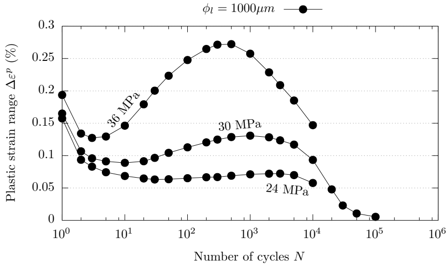
Figure 5: Evolution of \Delta\varepsilon^p during cycling for \phi_l , for different stress amplitudes.
