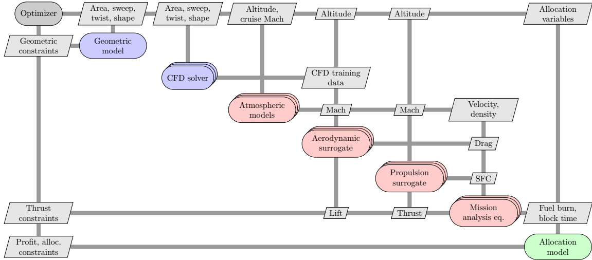
Figure 7: Extended design structure matrix [24] for the aircraft allocation-mission-design optimization problem that used RMTS [19]. The aerodynamic surrogate model predicts wing lift and drag coefficient as a function of the angle of attack, Mach number, and altitude. This surrogate model is retrained each iteration because the lift and drag training data change each optimization iteration as the aircraft wing design changes. Since a gradient-based algorithm is used for this large-scale optimization problem, we require output derivatives: derivatives of the lift and drag prediction outputs with respect to the lift and drag training data. These are provided by RMTS.
