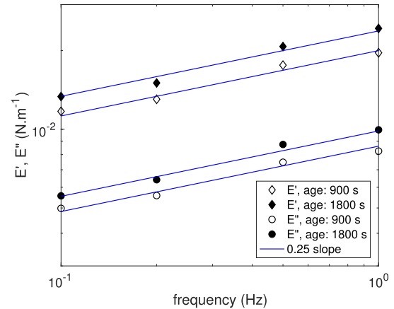
Figure 2. Evolution of interface moduli E' and E'' as a function of the frequency \omega/2\pi for two different ages within the first regime (900 and 1800 s).
