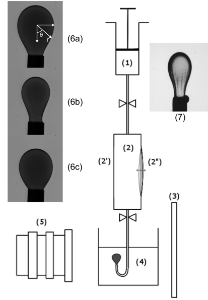
Figure 3. Experimental setup: (1) feeding syringe, (2) drop phase storing cell, (2') glass window, (2'') piezoelectric membrane, (3) LED backlight panel, (4) droplet formed at the tip of capillary tube immersed in water stored in a parallelepipedic optical-grade glass cell, (5) high-speed camera; (6) T2B interface before compression (a) after shrinkage (b) and just before oscillations (c). (7) Visualization of wrinkles on a shrunk interface.
