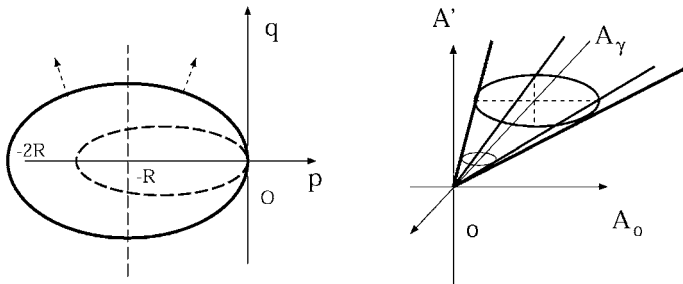
Fig. 3. Cam-clay model of geomaterials: the elastic domain is limited by a family of ellipses in the stress space ( p \times q ) and represented by a cone in the force space ( A_0 \times A' \times A_\gamma ).
