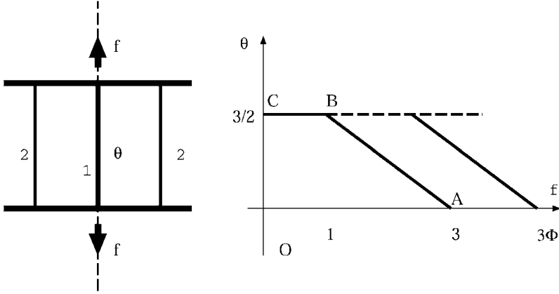
Fig. 4. A symmetric three-bar system and shakedown domains in perfect plasticity, limited kinematic hardening and linear kinematic hardening.
