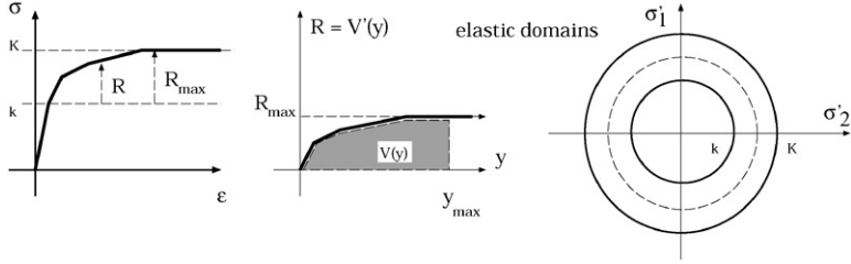
Fig. 1. A model for isotropic hardening.
