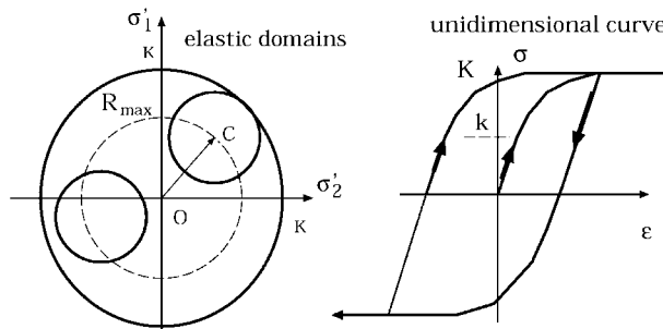
Fig. 2. A model for limited kinematic hardening.
