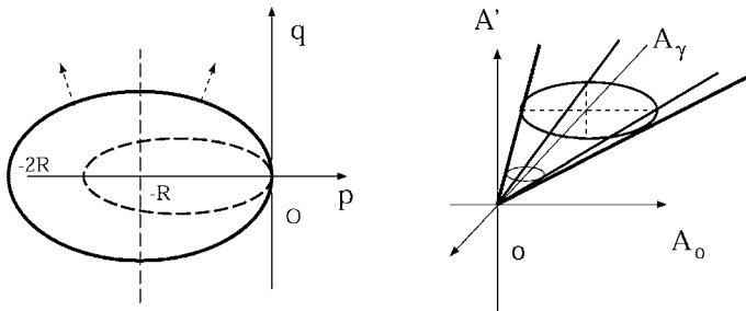
Fig. 3. Cam-clay model of geomaterials: the elastic domain is limited by a family of ellipses in the stress space ( p \times q ) and represented by a cone in the force space ( A_0 \times A' \times A_\gamma ).
