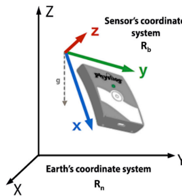
Figure 2. Earth and sensor’s coordinate systems.
