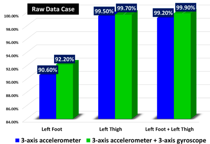
Figure 10. Comparison between the use of three-axis accelerometer raw data and the addition of three-axis gyroscope one in the case of static activities.
