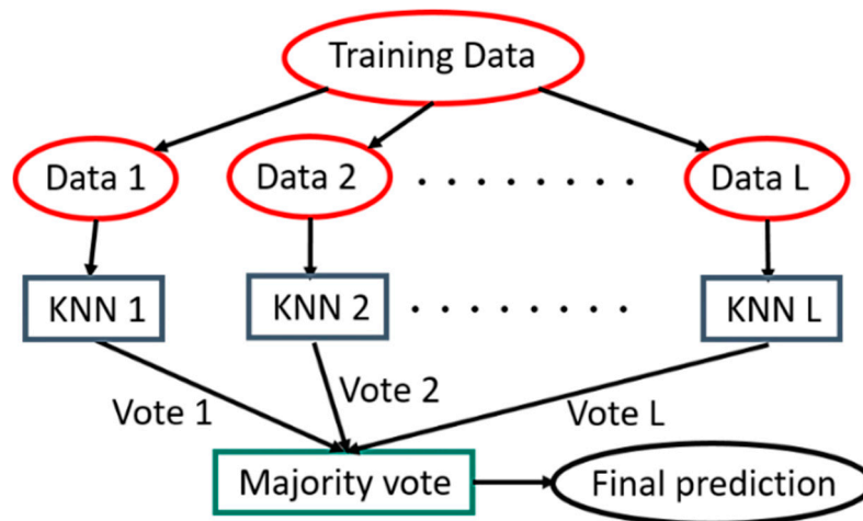
Figure 8. Subspace KNN architecture.
