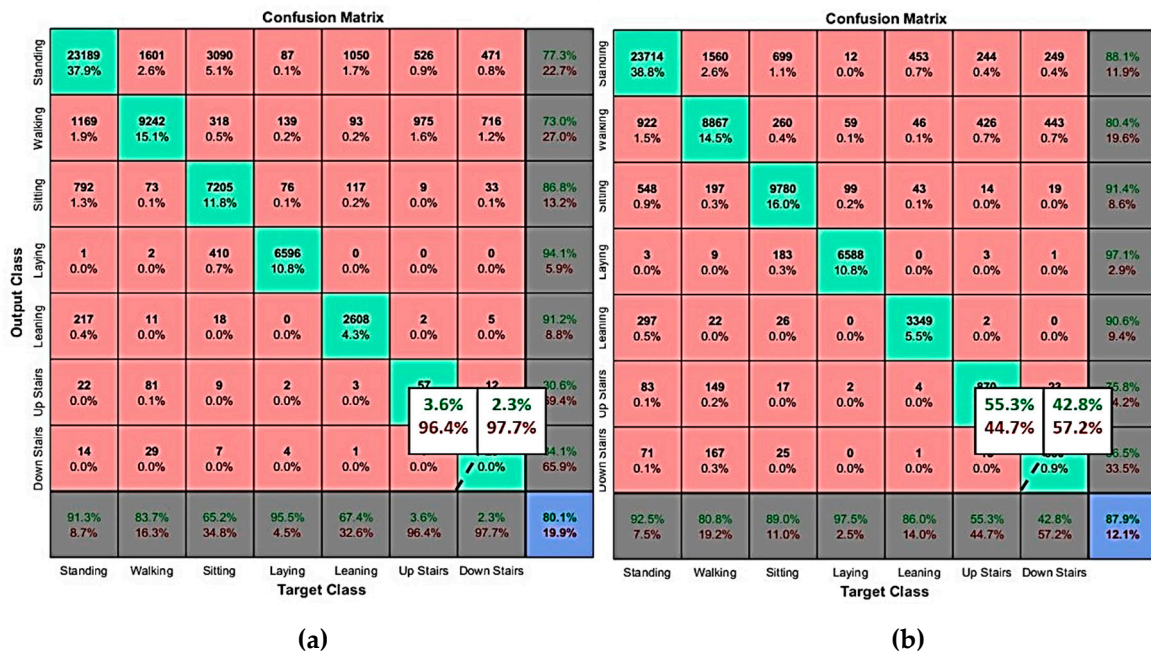
Figure 12. (a) Classification with raw data; (b) Classification with quaternion.
