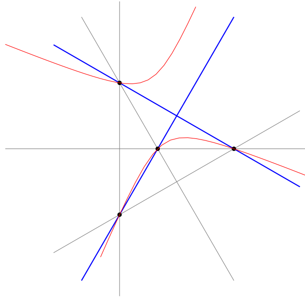
Figure 2: The pencil of conics. A generic fiber in red and one of the 3 singular fibers in blue.
