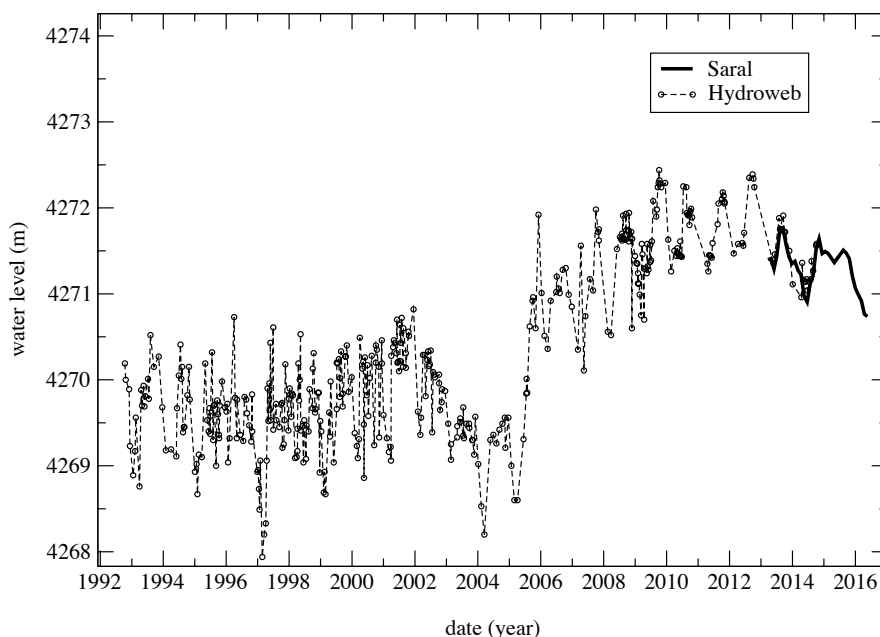
Figure 21. Water level change of Ngoring-Co Lake from a multi-satellite data processing. The lake was at equilibrium between 1992 and 2005 and has suddenly grown since 2006 to reach in a short time a new equilibrium, which slightly decreased after 2013 (extracted from Hydroweb database http://hydroweb.theia-land.fr/ and from SARAL/AltiKa data processing for the period 2013–2016).
