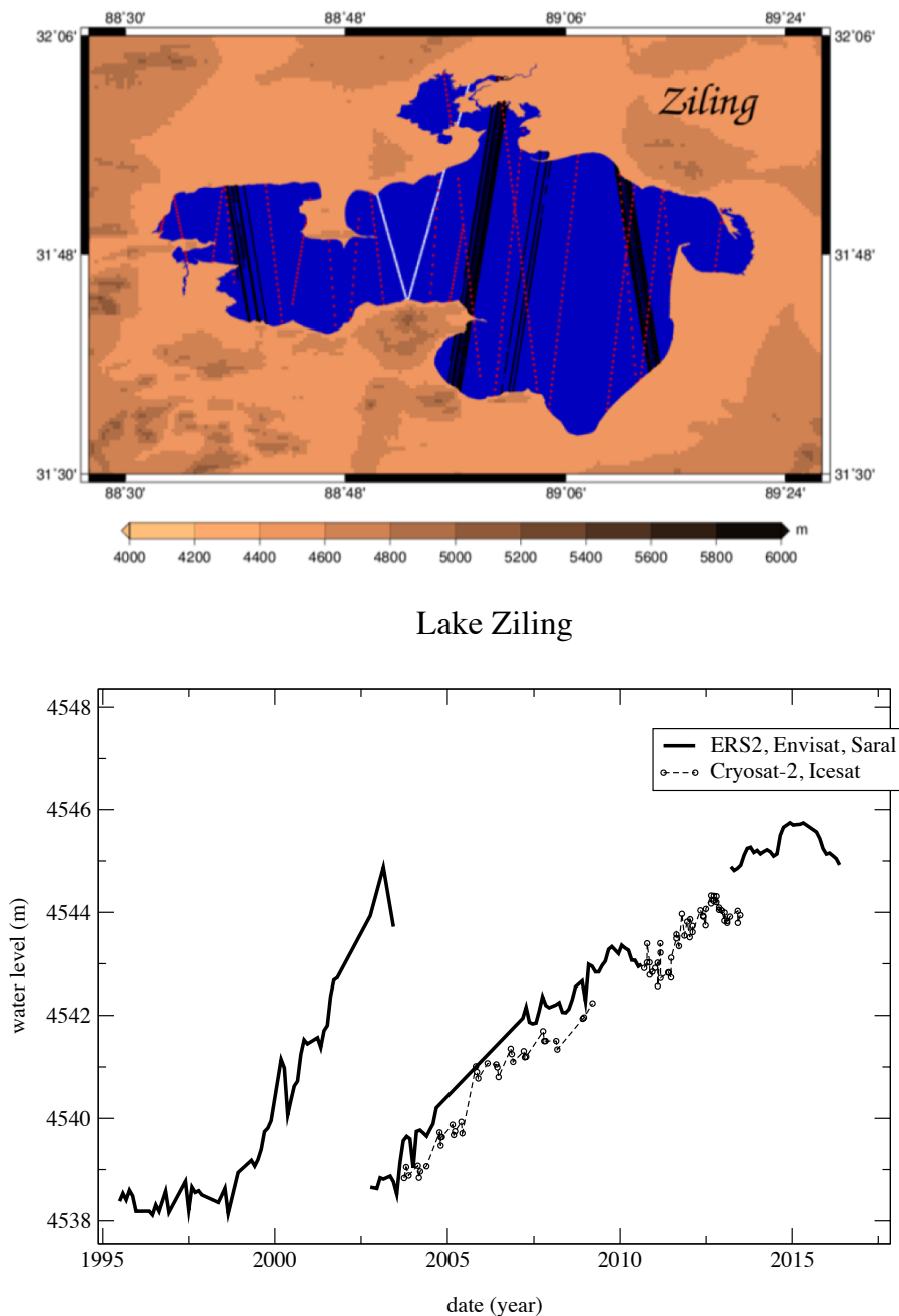
Figure 18. Tracks of satellite altimeters (black: ICESat; red: CryoSat-2; and white: ERS-2, Envisat and SARAL/AltiKa) over the Ziling Lake, one of the largest of the Tibetan Plateau (top); and water level changes from each satellite before correcting from inter-satellite tracks from 1995 to 2016 (bottom).
