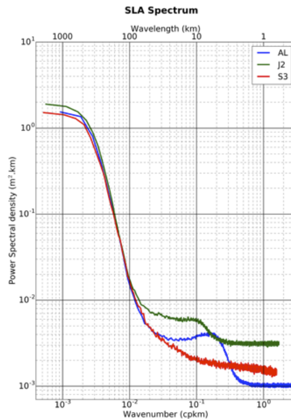
Figure 1. Globally-averaged wavenumber spectra of SSH anomalies (in \text{m}^2/\text{cpkm} ) from the highest resolution along-track data for three different missions: Jason-2 20 Hz (J2 in green); SARAL/AltiKa 40 Hz (AL in blue); and Sentinel-3 20 Hz SAR (S3 in red). The spectral “bump” in Jason-2 and SARAL/AltiKa data is due to surface roughness inhomogeneities within the footprint, mainly from surface waves.
