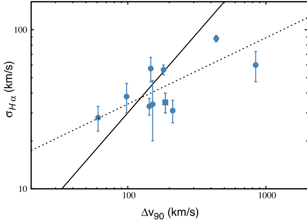
Figure 2. The velocity width of low-ion absorption lines, \Delta v_{90} , versus the velocity width of bright emission lines, \sigma_{\text{H}\alpha} , for 10 GRB host galaxies. The dotted line shows the best-fitting line when fitted together with the data presented in Fig. 1 (see Section 3 for details). The solid line ( \Delta v_{90} = 3.29 \sigma_{\text{H}\alpha} ) shows the relation between the two velocities if the absorption and emission profiles were identical. Note that the definition of the two velocity widths is different from each other: \sigma_{\text{H}\alpha} is the standard deviation of the fitted Gaussian function to the emission line while \Delta v_{90} is the velocity interval that contains 90 per cent of the area under the apparent optical depth. Hence, if the emission and absorption profiles were identical, the two velocity widths would not be identical but relate to each other as \Delta v_{90} = 3.29 \sigma_{\text{H}\alpha} . The host galaxy of the ultralong GRB 111209A is marked with a square.
