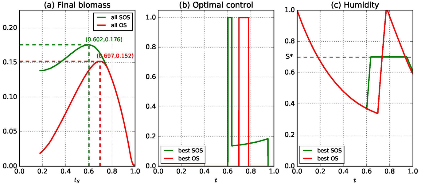
Fig. 2. Comparison of OS and SOS controls strategies on one typical example. Model parameters used are given in Table 1.
