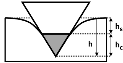
Fig. 5. Schematic representation of a section during indentation.
