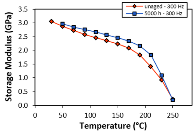
Fig. 7. Dynamic mechanical analysis of aged (for 5000 h) and unaged epoxy resin.
