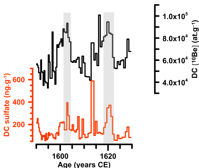
Figure 4. Period: 1590–1630 CE. ^{10}\text{Be} and sulfate concentrations from Dome C, shown as a function of time
