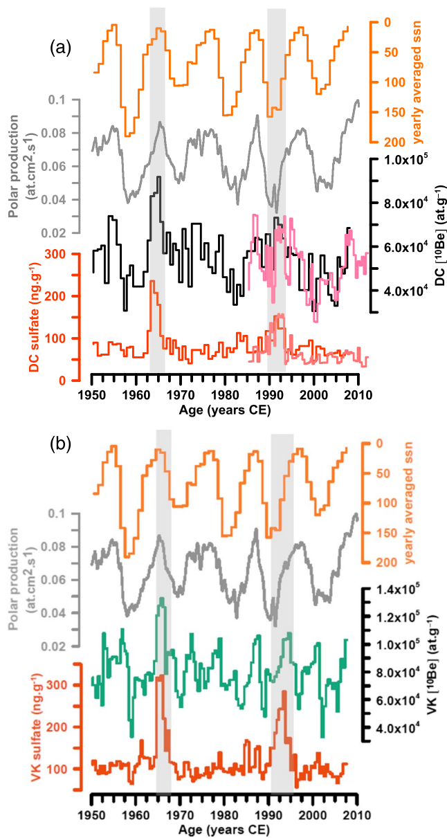
Figure 1. Period: 1950–2010 CE. ^{10}\text{Be} and sulfate concentrations, shown as a function of time (a) at Dome C (DC) and (b) at Vostok (VK) (a) ^{10}\text{Be} concentration from the Dome C ice core and from the Dome C snow pit are shown in black and pink, respectively. When available, solar proxies are represented for comparison. Polar ^{10}\text{Be} production from Poluianov et al. (2016) is shown for the 1950–2010 CE period covering the neutron monitor era. Yearly averaged sunspot numbers are represented from 1950 CE to 2010 CE ( http://www.sidc.be/silso ).
