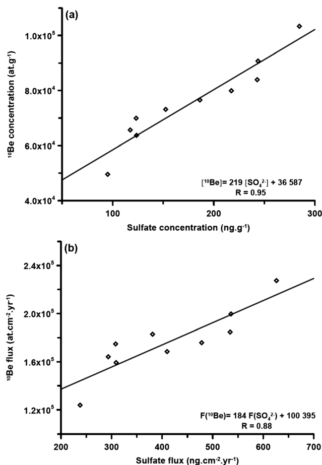
Figure 8. Linear regressions for Pinatubo based on merged data from Dome C and Vostok, given for (a) the ^{10}\text{Be} and sulfate concentrations ( [^{10}\text{Be}] = 219 (\pm 25)[\text{SO}_4^{2-}] + 36,587 (\pm 4,770) ) and (b) the ^{10}\text{Be} and sulfate fluxes ( F(^{10}\text{Be}) = 184 (\pm 36)[\text{SO}_4^{2-}] + 100,395 (\pm 15,419) ).
