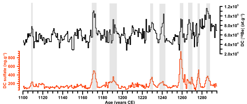
Figure 6. Period: 1100–1295 CE. ^{10}\text{Be} and sulfate concentrations from Dome C, shown as a function of time.
