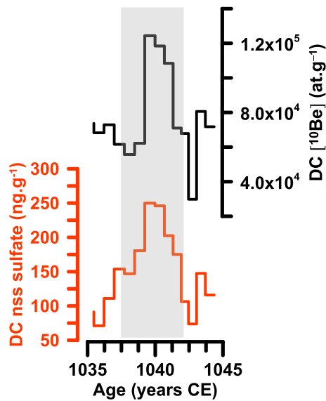
Figure 7. Period: 1035–1045 CE. ^{10}\text{Be} and sulfate concentrations from Dome C, shown as a function of time.
