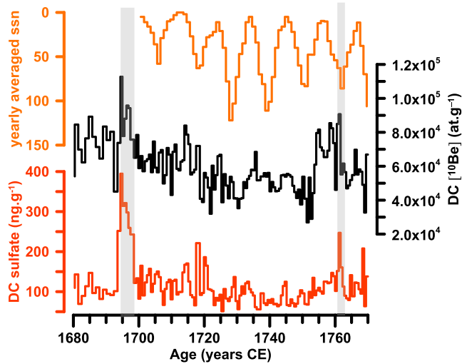
Figure 3. Period: 1680–1770 CE. ^{10}\text{Be} and sulfate concentrations from Dome C, shown as a function of time. Yearly averaged sunspot numbers are represented from 1700 CE to 1770 CE ( http://www.sidc.be/silso ).
