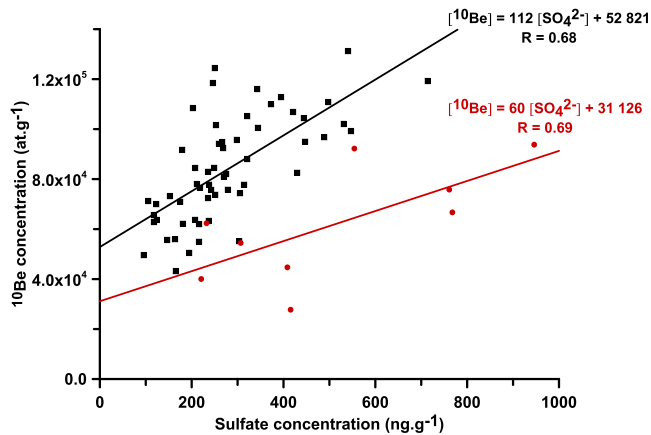
Figure 9. ^{10}\text{Be} concentration as a function of sulfate concentration for the nine volcanic eruptions exhibiting significant correlation between these proxies (Table 1, “significance” column), for the Dome C site (black squares). The 1269 UE is not taken into account (see section 3.4.). The equation of the corresponding line is [^{10}\text{Be}] = 112 (\pm 16)[\text{SO}_4^{2-}] + 52,821 (\pm 4,990) . The red dots correspond to the Samalash volcanic eruption in 1257 CE (Lavigne et al., 2013) recorded at Dome C: the equation is [^{10}\text{Be}] = 60 (\pm 24)[\text{SO}_4^{2-}] + 31,126 (\pm 13,626) (Table 1). UE = unknown event.
