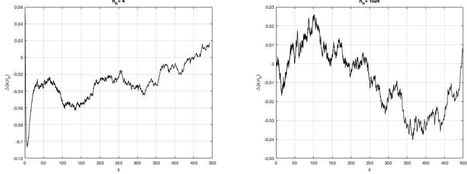
Figure 1: Log-tail approximation errors \Delta(x; n_h) for n_h = 4 and n_h = 1024 .
