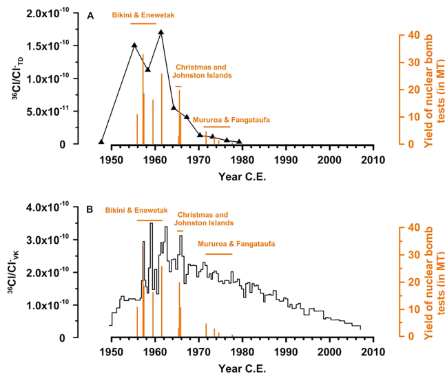
Figure 6. ^{36}\text{Cl}/\text{Cl}^- ratio for Talos Dome (a) and Vostok (b) records in comparison with nuclear marine bomb tests expressed in MT (see Table 1). We calculated the sum of the yields when different tests occurred in the same year. All the tests referenced have yields above 100 kT. The emission dates were shifted by 3 years from the emission time referenced in Table 1, to take into account the estimated 3 year residence time of ^{36}\text{Cl} in the stratosphere prior to deposition in the Antarctic snow (Heikkila, Beer, Feichter, Alfimov, et al., 2009). Only 10 of the 13 Talos Dome data points are reported in the upper panel, which focusses on the 1950–2010 period to enable better visualization of the nuclear bomb period.
