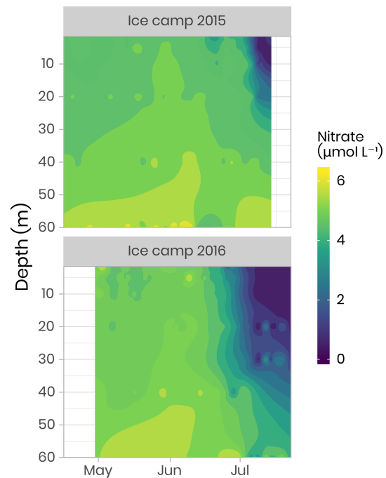
Figure 8. Temporal evolution of nitrate concentrations in the first 60 m of the water column for both ice camp missions.
