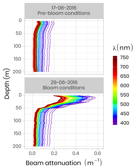
Figure 7. Beam attenuation coefficients ( c , m^{-1} ) measured in 2016 using a WetLabs AC-S before and during the phytoplankton bloom. Note that the colors of the lines correspond to wavelength frequencies.
