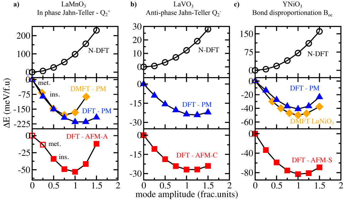
Figure 5: Energy gains \Delta E (in meV/f.u with respect to the 0-mode amplitude) associated with Jahn-Teller distortions (a and b) and the bond disproportionation (c) modes as obtained by the naïve nonmagnetic N-DFT (black circles, upper panel), the PM described with a SQS supercell (blue triangles, middle panel) and AFM (red squares, lower panel). DMFT potential (orange diamonds) for the PM phase of \text{LaMnO}_3 and \text{LuNiO}_3 extrapolated from Refs. 15,65 are also reported. Filled and unfilled symbols correspond to insulating (ins.) and metallic (met.) solutions. The reference structure at 0 amplitude of JT or B_{oc} modes is set to a material displaying octahedra rotations and anti-polar motions of ions.
