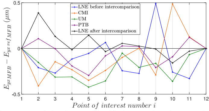
Figure 10: Deviation between identified E_{yx \text{ MFB}} the reference values.
