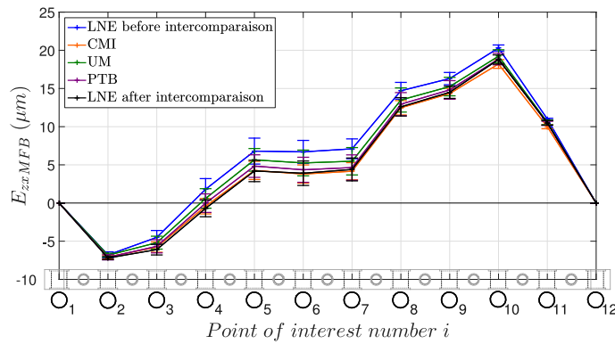
Figure 8: Vertical straightness error E_{zx \text{ MFB}} .
