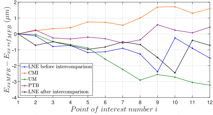
Figure 9: Deviation between identified E_{xx \text{ MFB}} and the reference values.
