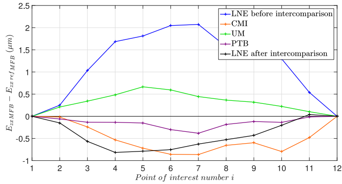
Figure 11: Deviation between E_{zx \text{ MFB}} and the reference values E_{zx \text{ MFB}} .
