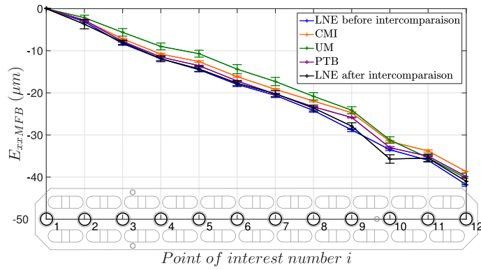
Figure 6: Linear positioning error E_{xx \text{ MFB}} .
