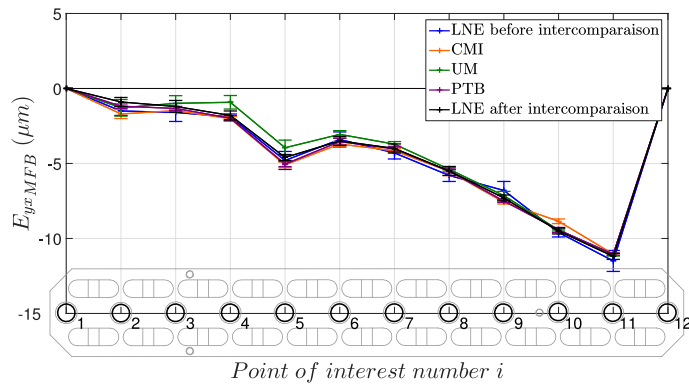
Figure 7: Horizontal straightness error E_{yx \text{ MFB}} .
