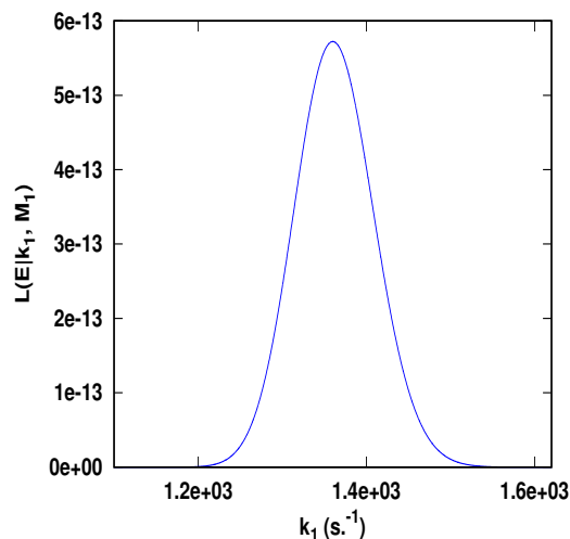
Figure 4: Likelihood ( M_1 )
