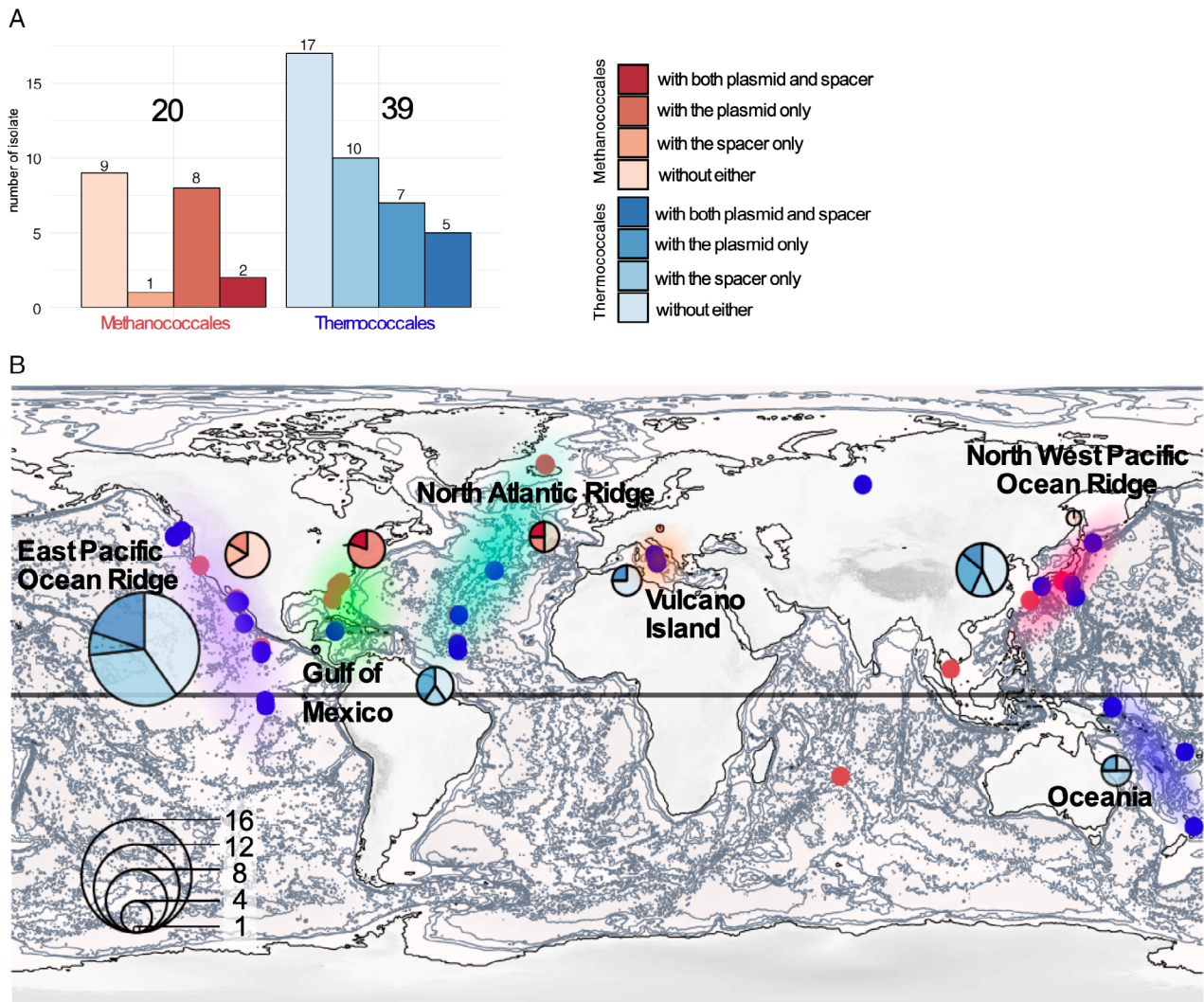
Fig. 1. Biogeography of the Thermococcales and Methanococcales isolation sites of the NCBI available genomes.
