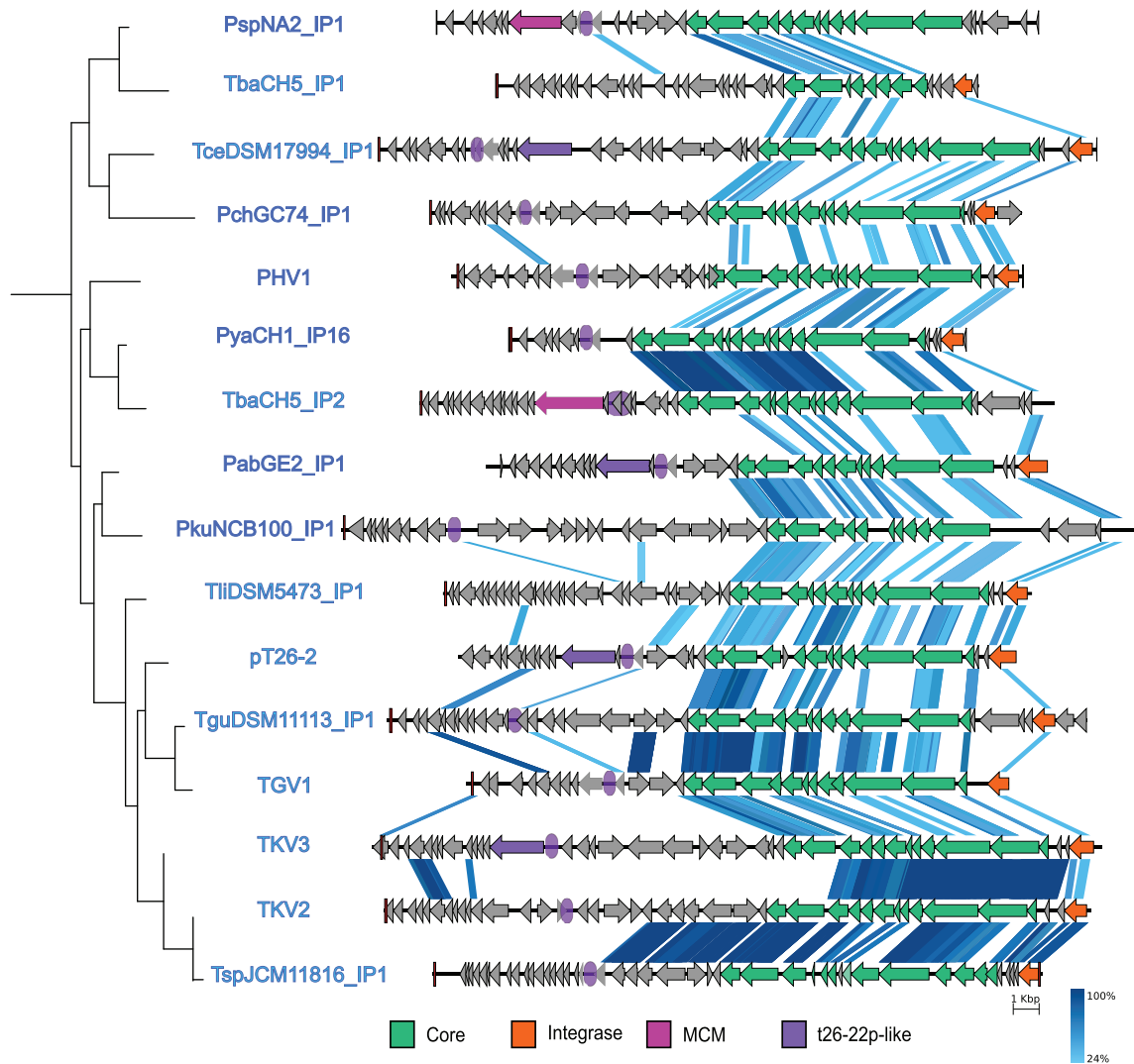
Fig. 3. Comparison of Thermococcales plasmids of the pT26-2 family.
