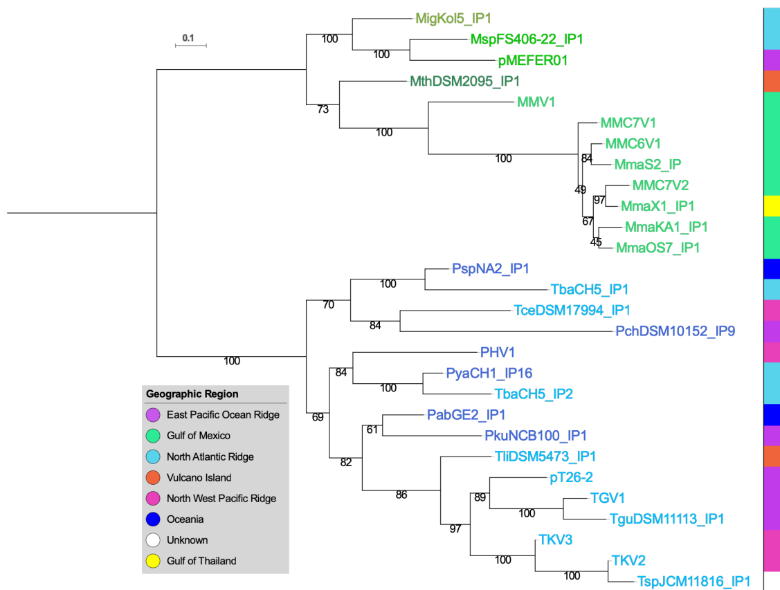
Fig. 5. Maximum likelihood tree of the concatenated CORE proteins. The isolation region is indicated by a coloured square. The scale-bars represent the average number of substitutions per site. Values at nodes represent support calculated by nonparametric bootstrap (out of 100).
