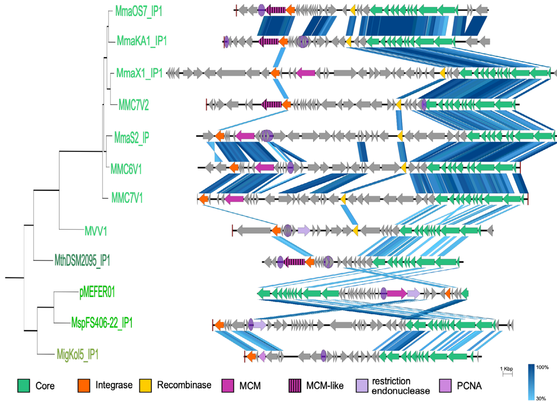
Fig. 4. Comparison of Methanococcales plasmids of the pT26-2 family.
