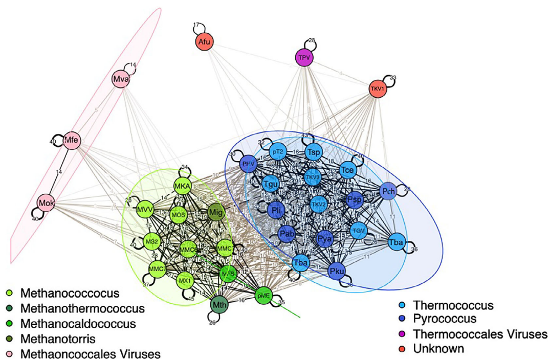
Fig. 2. Network view of plasmids of the pT26-2 family conservation.
