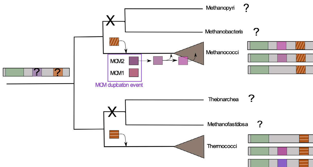
Fig. 7. The evolutive model of the pT26-2 family. In this schematic representation, the core module and the integrase module are indicated in green and orange respectively. The different replication modules are indicated with different shade of purple.
