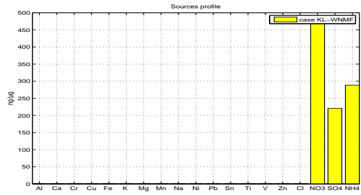
Fig. 2. Secondary inorganic aerosols
