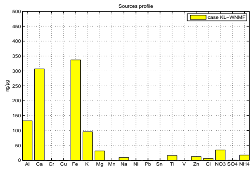
Fig. 3. Intermediate profile between crustal source and blast furnaces-steel plant source.
