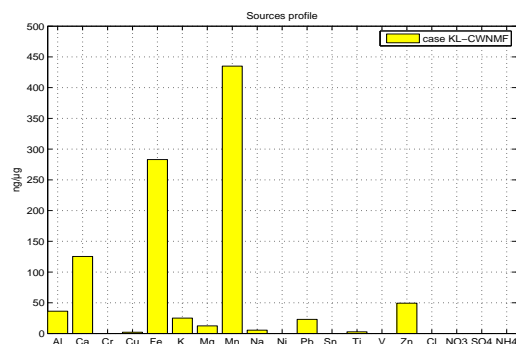
Fig. 8. KL-CWNMF: Ferromanganese alloys profile
