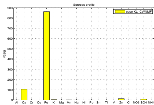
Fig. 4. KL-CWNMF: Blast furnaces - steel plant profile
