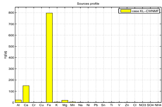
Fig. 6. KL-CWNMF: Ores sintering profile
