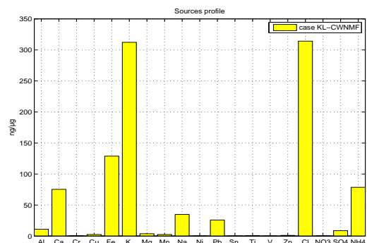
Fig. 7. KL-CWNMF: Sintering chimney profile
