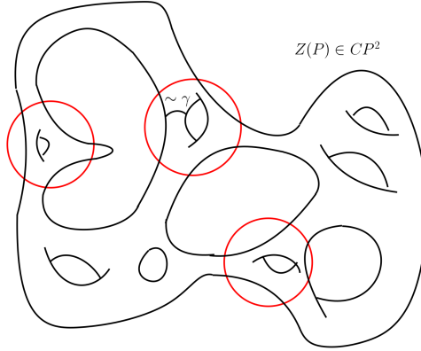
Figure 4: A (nonrealistic) degree 6 curve in \mathbb{C}P^2 and three small balls of size 1/\sqrt{d} containing the affine complex curve \Sigma and the non-trivial real curve \gamma of Figure 3.
