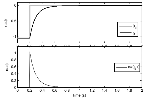
Figure 4: step response on \theta .
