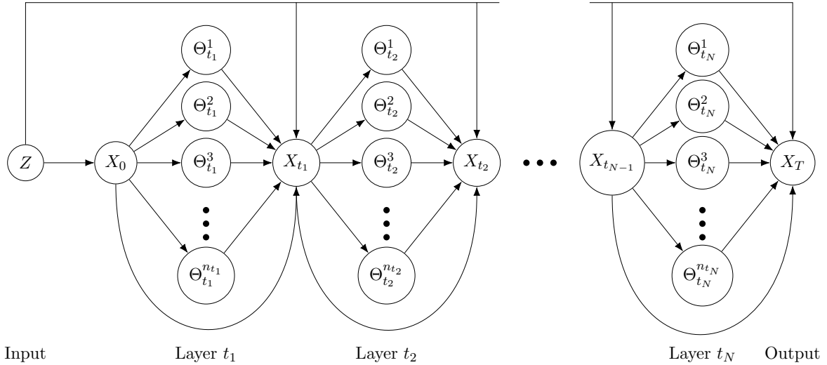
Neural network corresponding to the relaxed controlled process
