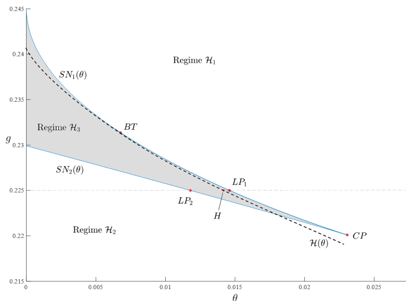
Figure 7: Location of regimes and bifurcation points in the (\theta, g) plane
