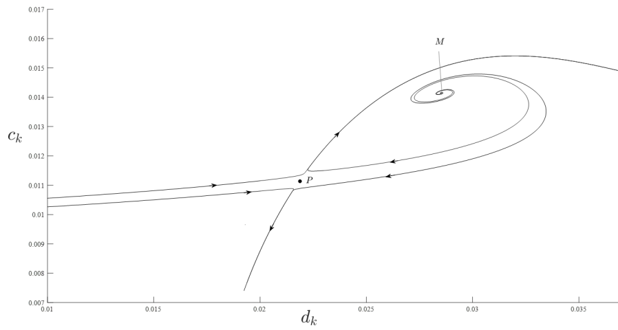
9d: Limit-cycles vanish ( \theta < \tilde{\theta} )
