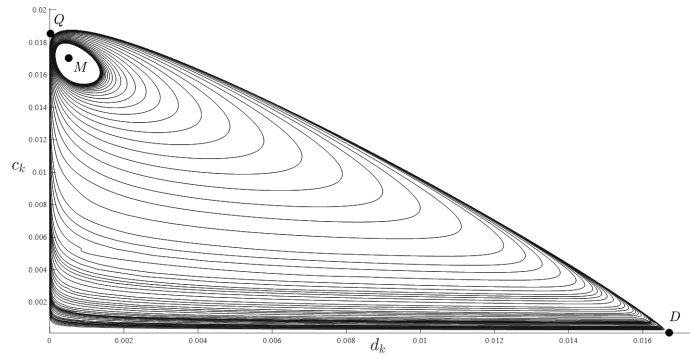
12a: The family of periodic orbits as g increases
