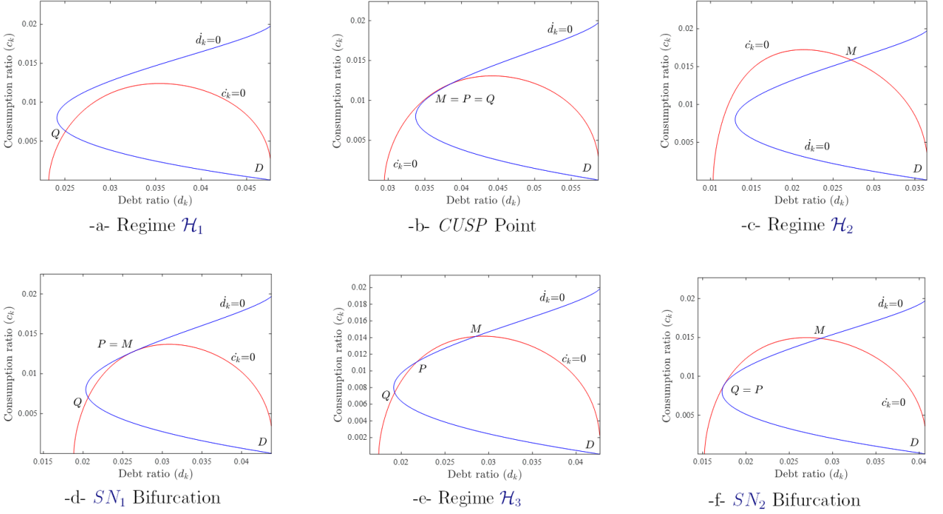
Figure 4: Topological regimes in Regime \mathcal{H} ( \hat{c}_k < \bar{c}_k )
