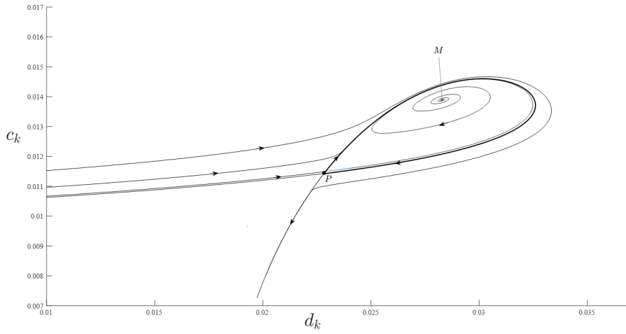
9c: Saddle-loop bifurcation ( \theta = \tilde{\theta} )
