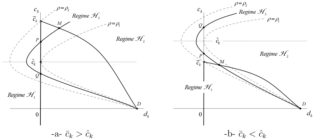
Figure 11: Topological behaviour of Regime \mathcal{H} ( \theta = 0 )
