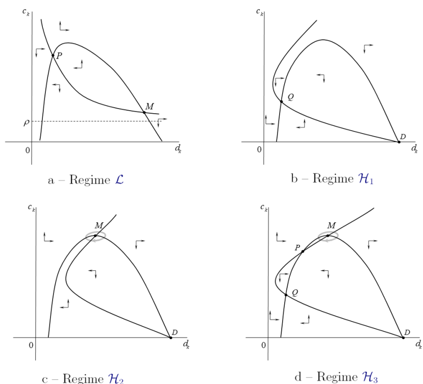
Figure 6: Global dynamics
