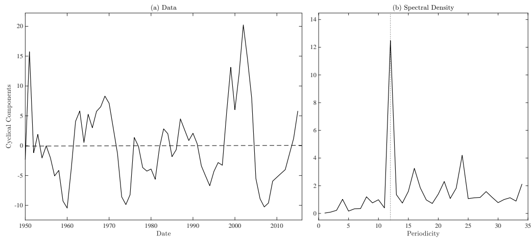
Figure 2: Cyclical Component and Spectral Densities for Developing Countries
