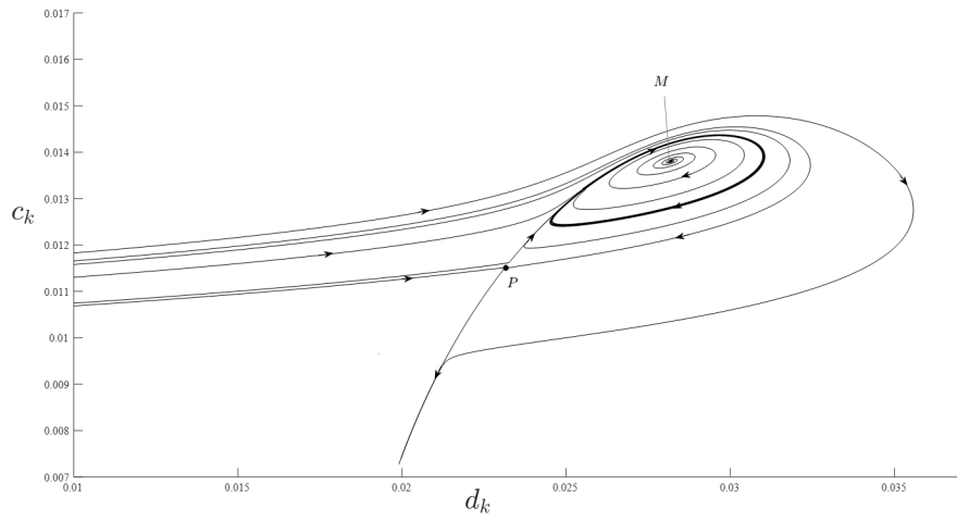
9b: Stable limit cycle around M ( \tilde{\theta} < \theta < \theta^h )
