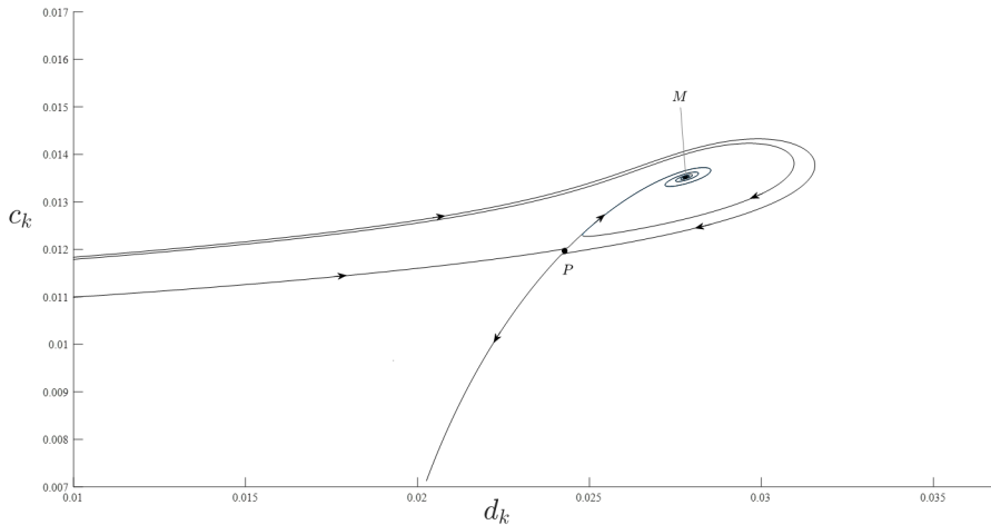
9a: M is stable ( \theta^h < \theta )
