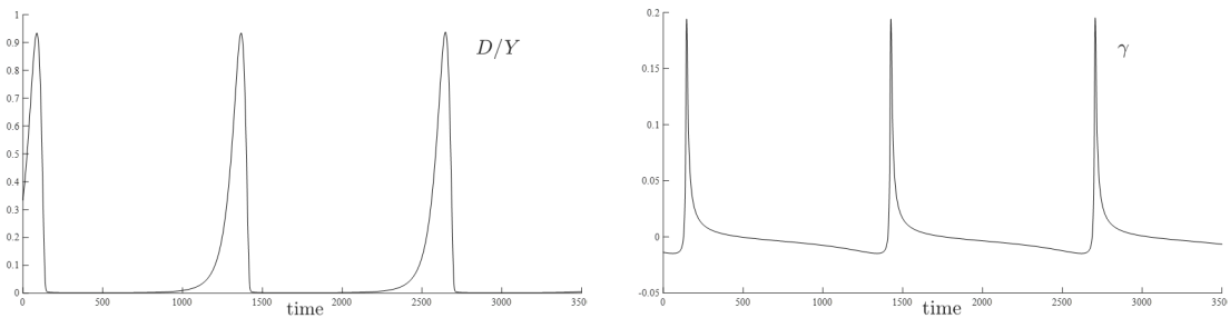
12b: Behavior of the debt ratio and economic growth for g = 0.2348
