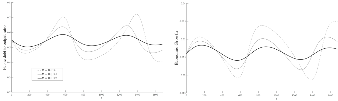
Figure 8: Public debt and growth cycles as a function of \theta
