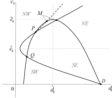
Figure A1: Local stability ( \hat{c}_k < \bar{c}_k )
