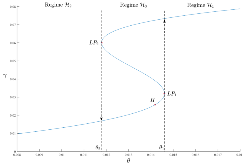
Figure 5: Bifurcation diagram as a function of \theta (regime \mathcal{H} )
