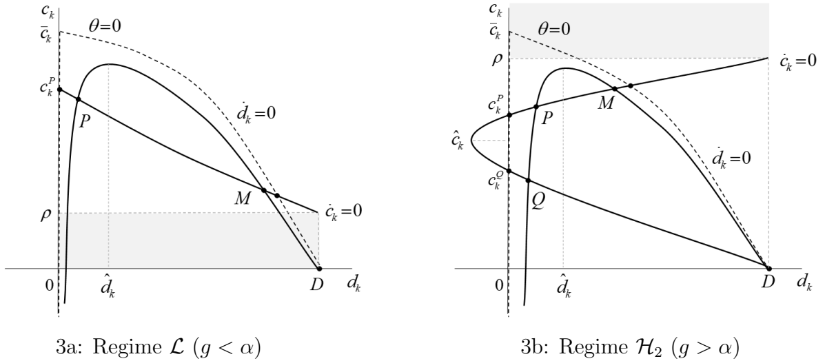
Figure 3: The steady states
