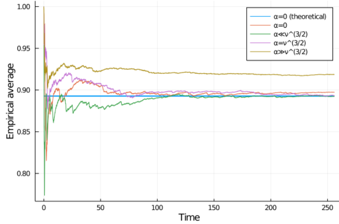
FIGURE 1. Evolution of \widehat{I}_t^{N,\Delta t} for t \in [0, T] and the four regimes of \alpha . In the case \alpha = 0 , the theoretical value of I^{N,\Delta t} is superposed as a horizontal line. Here, N = 32 , \Delta t = 2^{-10} and T = 256 .
