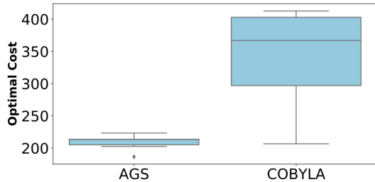
Fig. 6: Optimal cost function from unfeasible starting sets ( s_1, s_2, s_3, s_4, s_5, s_{all} ).
