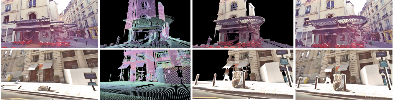
Figure 1: Rendering using mesh and pointCloud. a) Projective texturing on simplified planar geometry (point of view one meter distant from original photography position) b) Original Point cloud c) Projective texturing on Point Cloud. d) Hybrid rendering.
