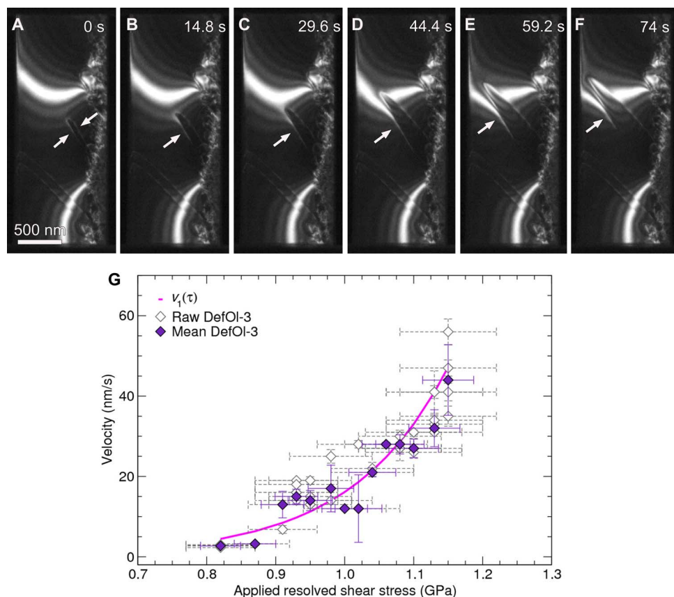
Fig. 3. TEM measurements of the mobility of screw dislocations. (A to F) Video frames captured during the in situ deformation of sample DefOl-3 under a constant load of 384 \mu\text{N} (resolved shear stress, 0.89 GPa). A movie is available in the Supplementary Materials. The loop expands from the scratch and develops, allowing propagation of the screw segment (arrowed) to be followed across the specimen. A table describing the different experiments is included in the Supplementary Materials. (G) Velocities (in \text{nm s}^{-1} ) of screw dislocations versus stress (in GPa). Data from the DefOl-3 experiment are presented for all raw measurements (empty diamonds) and weighted means at each stress (indigo diamonds). v_1(\tau) is the fit introduced in the DD model (see the Supplementary Materials). These velocities correspond to a screw dislocation segment of length 0.8 \mu\text{m} .
