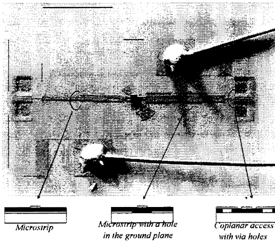
Fig. 3. Photograph of the multilayer frequency doubler. The surface is 6.7 mm x 9.7 mm.
