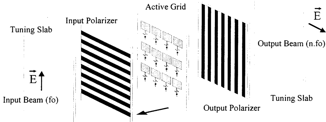
Fig. 5. Quasi-optical frequency multiplier.
