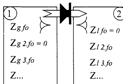
Fig. 1. Impedance optimization at each port.
