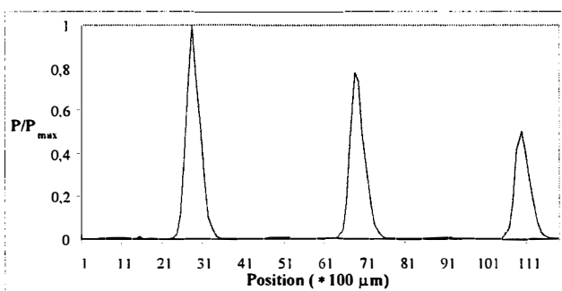
Fig. 8. Normalized output power measurement of the quasi-optical multiplier for different positions of the input polarizer in relation to the active grid.
