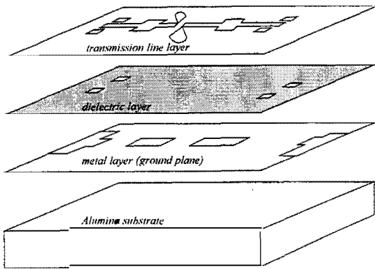
Fig. 2. Multilayer technology process on an Alumina substrate with two metal layers and one dielectric layer.
