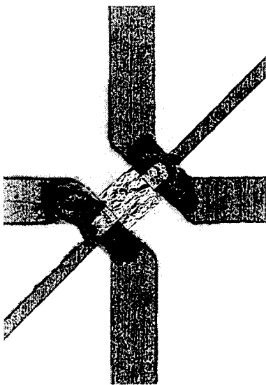
Fig. 7. Detail of the diode connected to dipole antennas.
