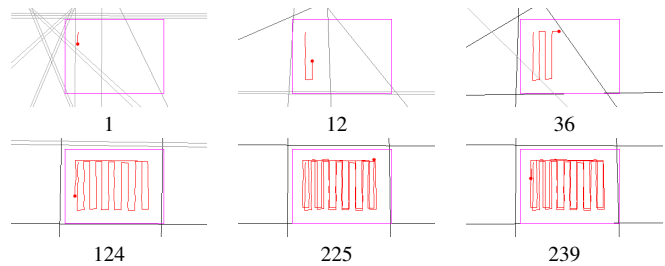
Fig. 6. Evolution of the map representation for the highest-ranked particle at step 1, 12, 36, 124, 225 and 239. The purple frame represent the outline of the true plate. The red dot is the current estimated sensor pose and the red line is the history of its estimated trajectory. The darkness of the line is proportional to the number of times they have been observed.
