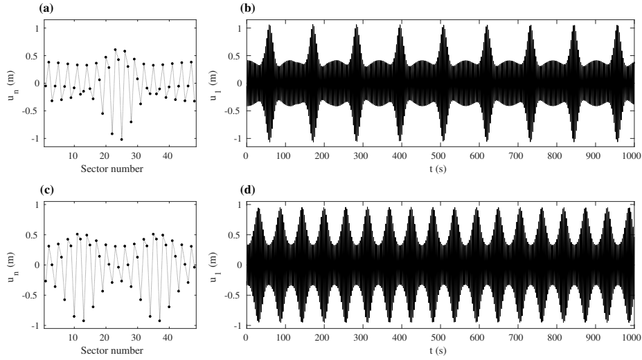
Figure 4: Results obtained through numerical time integration of the physical system for k=16 \text{ m}^{-1} and F_0=0.007 \text{ ms}^{-2} . Panel (a): the spatial displacements at t=0 \text{ s} calculated at P1 in Fig. 3; Panel (b): time-evolution of the displacement u_1(t) of the first oscillator. Panels (c) and (d) illustrate the same quantities for P2.
