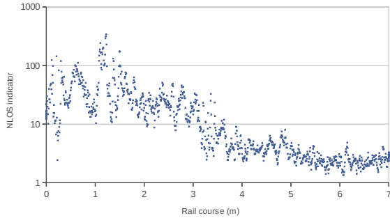
Fig. 9. NLOS Indicator vs. Rail Course
