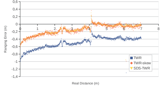
Fig. 7. Ranging Error vs Distance, for each protocol
