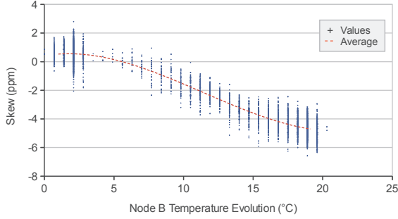
Fig. 5. Skew vs. Transceiver Temperature in Experiment #1
