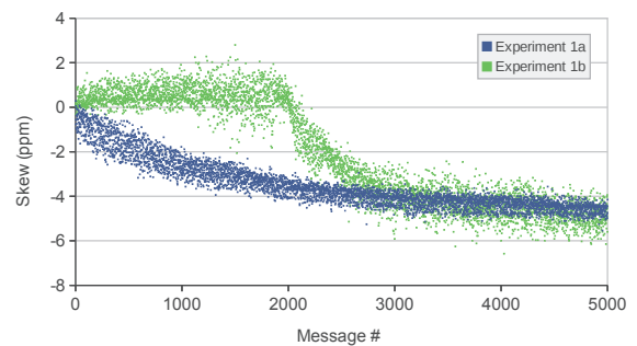
Fig. 4. Skew Evolution for experiment #1a and #1b
