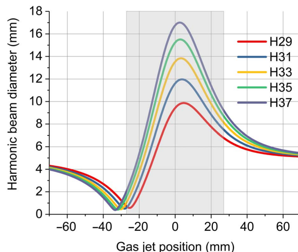
Fig. 3. Calculated diameters (FWHM) of the Gaussian XUV beams at a distance of 2.9 m after the IR focus position. The shaded area represents the zone where the jet is within the IR beam Rayleigh range.
