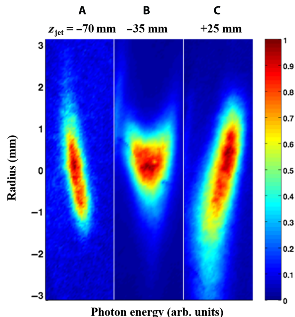
Fig. 4. Spatial chirp of harmonic 29. Far-field spatially resolved normalized spectra of the harmonic 29 generated in neon for three positions of the generating medium (A) z_{\text{jet}} = -70 mm, (B) z_{\text{jet}} = -35 mm, and (C) z_{\text{jet}} = +25 mm. HHG was performed with a fundamental beam that was spatially chirped in the generating medium. The tilt of the spatially resolved harmonic spectra is the signature of a spatial chirp in the XUV beam in the far field.
