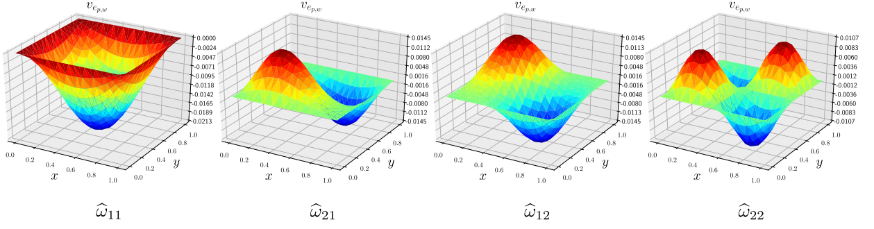
Fig. 5. Eigenvectors for the SSSS case.
