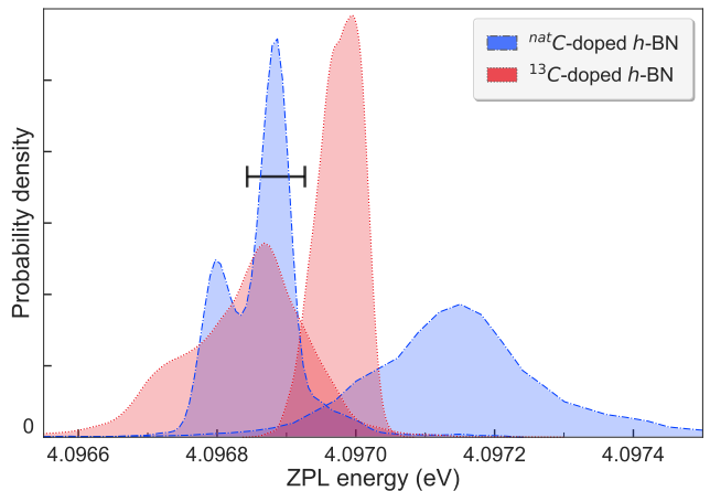
FIG. 6. Statistical analysis of the ZPL energy in ^{13}\text{C} - and ^{nat}\text{C} -doped hBN crystals: the normalized probability density of the ZPL energy is plotted for four 30\times30\text{ }\mu\text{m}^2 regions; two in a ^{13}\text{C} -doped crystal (C40, red data), two in a ^{nat}\text{C} -doped crystal (C27, blue data). The 100\text{ }\mu\text{eV} -large horizontal bar indicates the difference of the mean values of the ZPL energy in ^{13}\text{C} - and ^{nat}\text{C} -doped hBN crystals, the mean values being calculated for a total of ten 30\times30\text{ }\mu\text{m}^2 regions.
