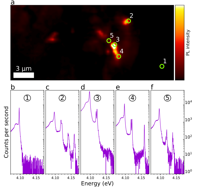
FIG. 10. (a) Spatial variations of the PL signal intensity recorded by a UV scanning confocal microscope in sample C27, at 10 K, for an excitation power of 0.35 mW. The PL signal is integrated from 4.112 to 4.175 eV. 5 s integration time per acquisition point. (b-f) PL spectrum on a log scale recorded at the five different locations indicated by circles in (a).
