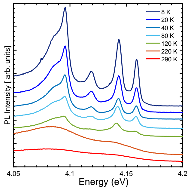
FIG. 8. Temperature-dependent PL measurements (linear scale) in the heavily carbon-doped hBN sample C33, in the 4.05 to 4.2 eV range. The spectra are vertically shifted for clarity.
