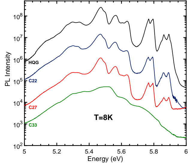
FIG. 3. PL spectra recorded at 8 K in bulk hBN crystals for energies ranging between 5 and 6 eV (semi-log scale). Spectra are vertically shifted for clarity. Growth conditions are given in Table 1. HQG stands for a test un-doped hBN crystal purchased from HQ Graphene.
