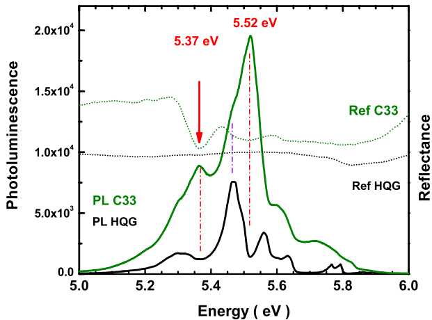
FIG. 4. PL (solid lines) and reflectance (dotted lines) spectra on linear scales, recorded in a test un-doped hBN crystal (HQG, black lines) and a heavily carbon-doped one (C33, green lines) at 10 K. Note the coincidences between the reflectance minima and the PL maxima in sample C33.
