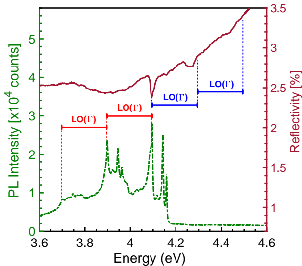
FIG. 9. PL (green dashed line) and reflectivity (purple solid line) spectrum on linear scales, recorded at 8K for sample C33 in the 4 eV region. The horizontal bars have a 200 meV width, corresponding to the \text{LO}(\Gamma) phonon energy. They are displayed in red for the red-shifted phonon-assisted emission (below 4.1 eV), and in blue for the blue-shifted phonon-assisted absorption (above 4.1 eV).
