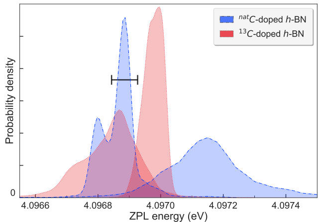
FIG. 6. Statistical analysis of the ZPL energy in ^{13}\text{C} - and ^{nat}\text{C} -doped hBN crystals: the normalized probability density of the ZPL energy is plotted for four 30\times 30\ \mu\text{m}^2 regions; two in a ^{13}\text{C} -doped crystal (C40, red data), two in a ^{nat}\text{C} -doped crystal (C27, blue data). The 100\ \mu\text{eV} -large horizontal bar indicates the difference of the mean values of the ZPL energy in ^{13}\text{C} - and ^{nat}\text{C} -doped hBN crystals, the mean values being calculated for a total of ten 30\times 30\ \mu\text{m}^2 regions.
