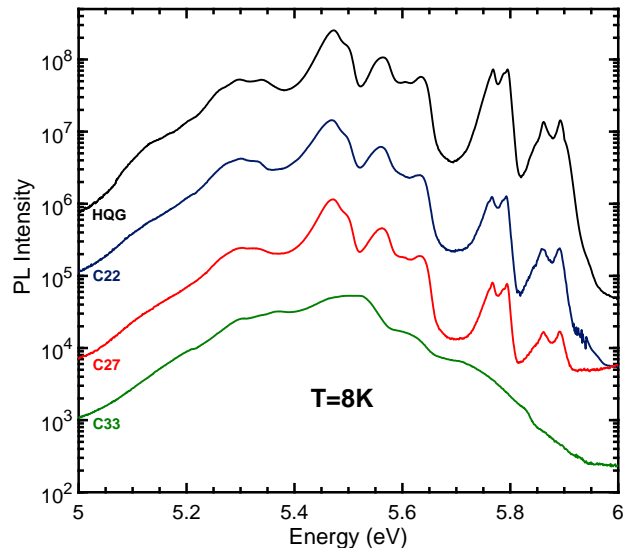
FIG. 3. PL spectra recorded at 8 K in bulk hBN crystals for energies ranging between 5 and 6 eV (semi-log scale). Spectra are vertically shifted for clarity. Growth conditions are given in Table 1. HQG stands for a test un-doped hBN crystal purchased from HQ Graphene.
