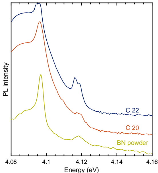
FIG. 2. Zoom in the 4 eV region (linear scale) of the macro-PL spectrum in bulk hBN synthesised either with iron (C20) or nickel (C22), together with a hBN powder used as precursor (BN Powder).
