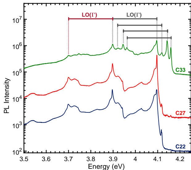
FIG. 7. Full set of the PL spectra (semi-log scale) of carbon-doped hBN samples in the 3.5 to 4.25 eV range. The spectra are vertically shifted for clarity. Note the occurrence of new lines at higher energy than 4.1 eV. The horizontal bars have a 200 meV width, corresponding to the LO( \Gamma ) phonon energy.
