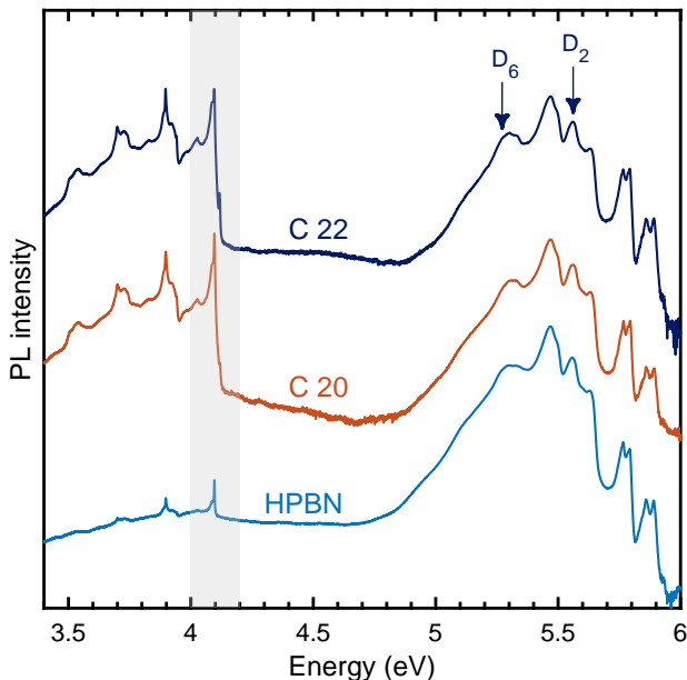
FIG. 1. Macro-PL spectrum at 8 K (semi-log scale), with an excitation energy of 6.35 eV, in bulk hBN synthesized either with iron (C22) or nickel (C20), and the hBN powder used as precursor, here in the form of Hot Pressed Boron Nitride (HPBN).
