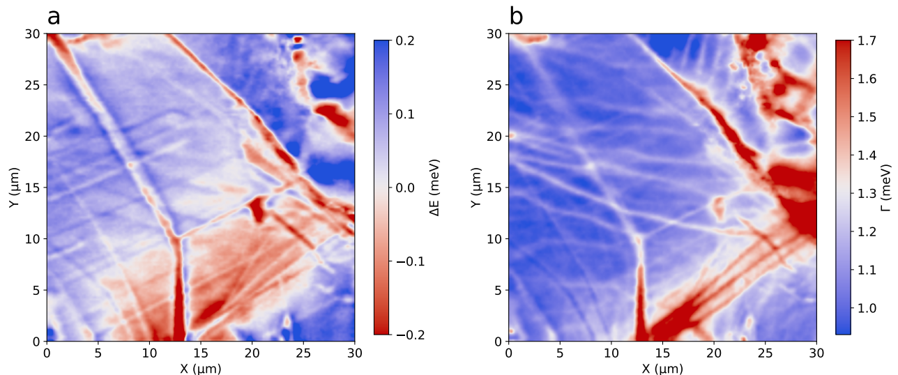
FIG. 5. Spatial variations of the shift \Delta E (a) and broadening \Gamma (b) of the ZPL in a 30 \times 30 \mu\text{m}^2 region of sample C40 at 10 K. The average ZPL energy is 4.0968 eV.
