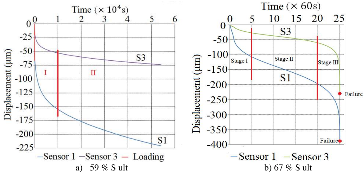
Fig. 9: Creep shear at T = 25^{\circ}\text{C} .
